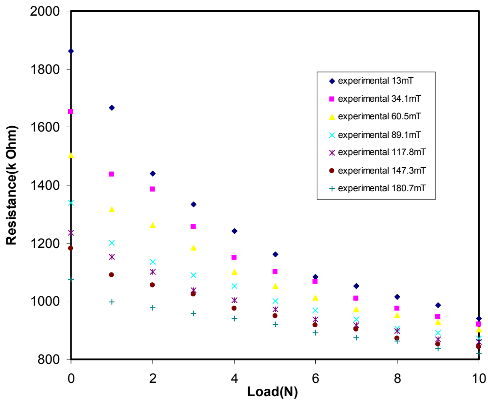
Figure 19. Resistance versus load (anisotropic MRE Gr 20%)
