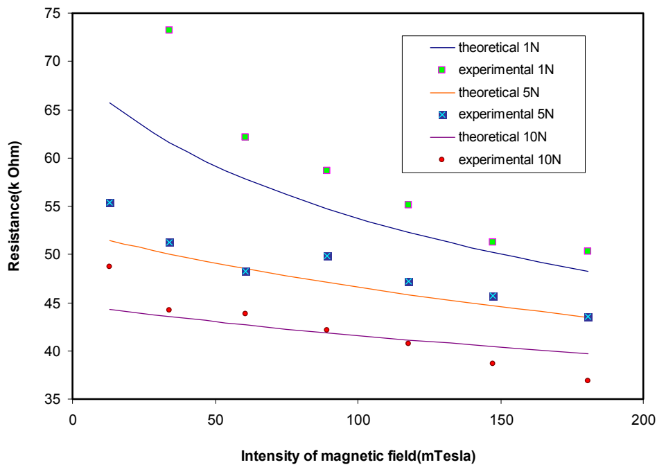
Figure 27. Resistance changing at a fixed load (anisotropic MRE Gr 21.95%)
