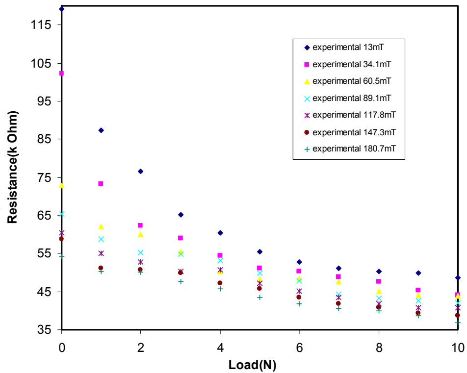
Figure 20. Resistance versus load (anisotropic MRE Gr 21.95%)
