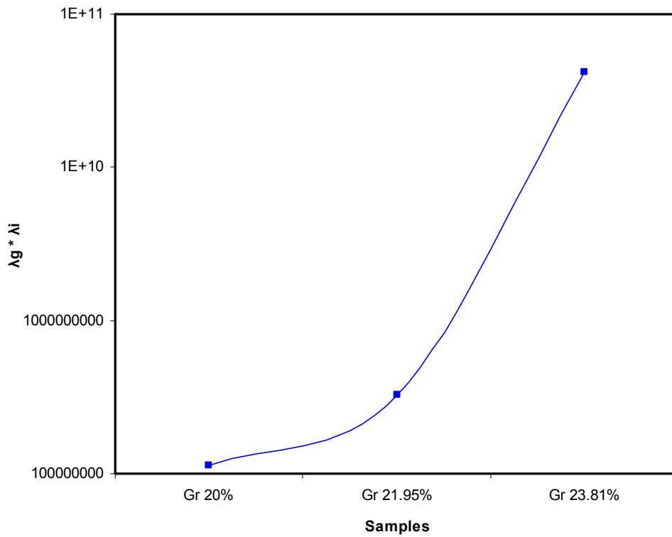
Figure 25. \lambda_g * \lambda_i versus graphite weight fraction
