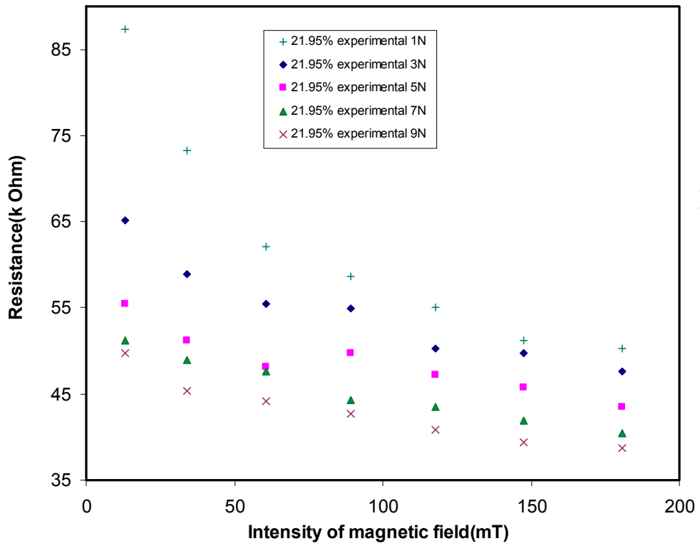
Figure 22. Resistance versus magnetic field (anisotropic MRE Gr 21.95%)
