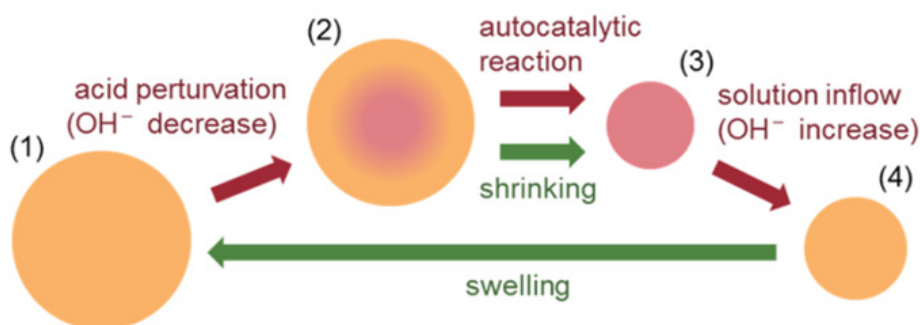
Figure 14. Flowchart of the chemical reaction networks. Each disk shows the condition of a spherical gel. The red areas indicate the acid steady state and the yellow areas indicate the alkaline steady state. There are four steps in the networks: (1) The spherical gel is in the uniform alkaline steady state. (2) When the gel radius grows and exceeds a certain threshold value, an acid perturbation rises in the core of the gel. (3) The acid region fills the gel entirely, and the gel shrinks. (4) When the gel radius shrinks below a certain threshold value, it swells again by inflowing of alkali solution.
