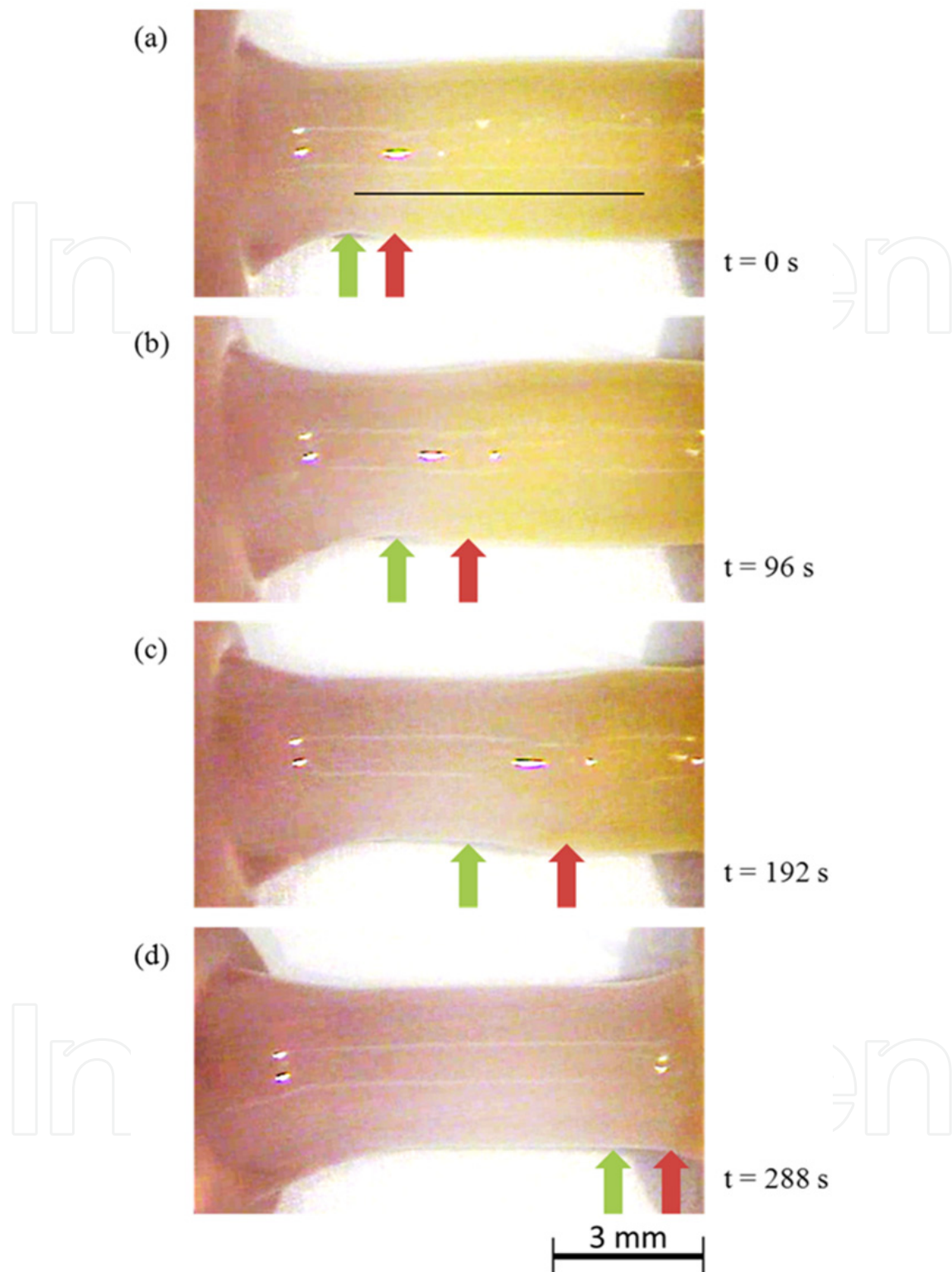
Figure 18. Propagation of the acid front in the swollen part of the tubular gel. An acid perturbation was applied to the left part of the gel. The yellow area corresponds to alkaline composition and the red area corresponds to acid composition. The red arrows indicate the forefronts of the acid regions and the green arrows indicate the forefronts of the gel contraction, which are the rightmost points obtained locally minimum diameters. (a) t = 0 indicates the criterion time after applying the acid perturbation. (Reprinted ref. 58, Copyright IEEE . Reproduced with permission.)
