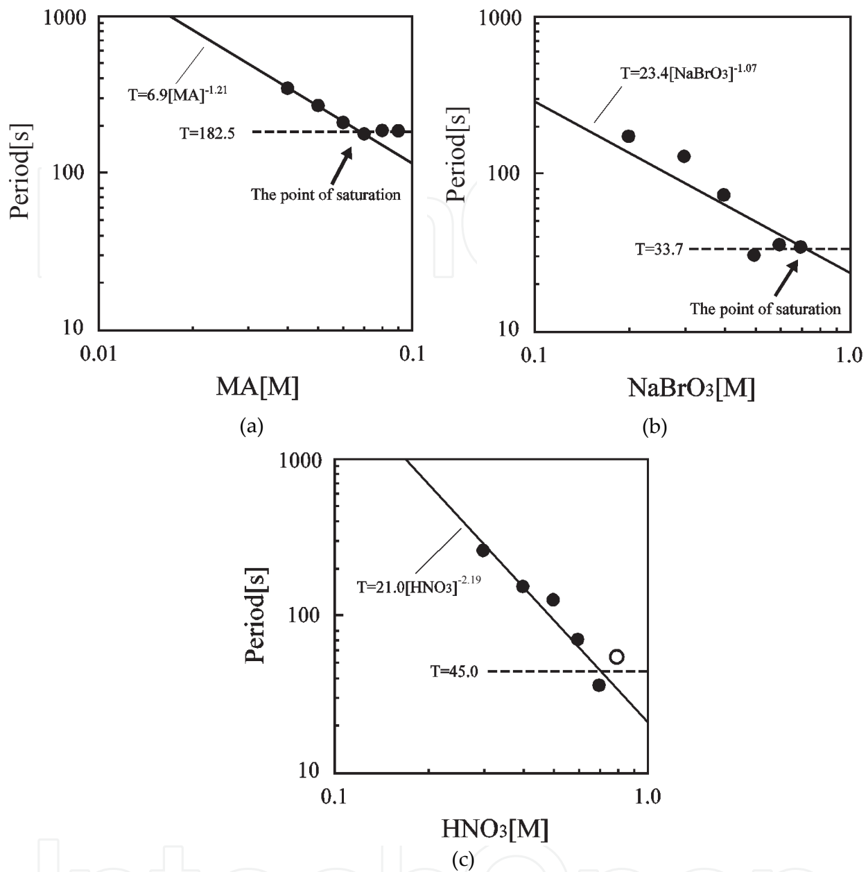
Figure 11. Logarithmic plots of period ( T in s) vs initial molar concentration of one BZ substrate at a constant temperature ( T=20\text{ }^{\circ}\text{C} ) under fixed concentrations of the other two BZ substrates; (a) [\text{NaBrO}_3] = 0.084\text{M} and [\text{HNO}_3] = 0.3\text{M} , (b) [\text{MA}] = 0.0625\text{M} and [\text{HNO}_3] = 0.3\text{M} , (c) [\text{MA}] = 0.0625\text{M} and [\text{NaBrO}_3] = 0.084\text{M} . (●) plots and (○) plots show the linear relation and the saturated line vs initial concentration of one BZ substrate, respectively. (Reprinted ref. 57, Copyright American Chemical Society. Reproduced with permission.)
