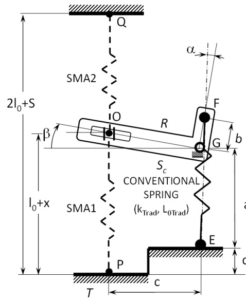
Figure 10. Oscillating rocker arm compensation mechanism
