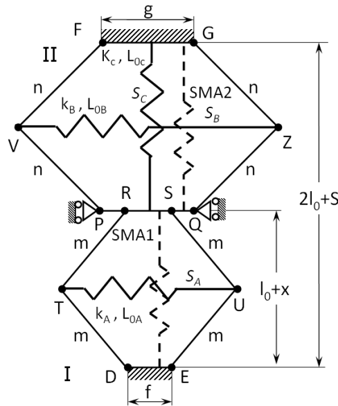
Figure 11. Double articulated quadrilateral compensation mechanism
