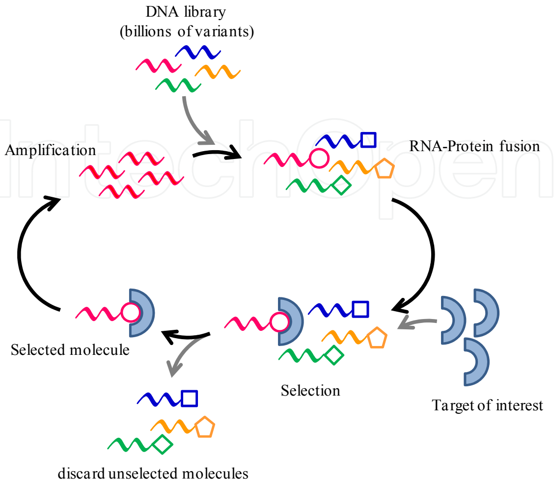
Figure 5. A schematic drawing of Directed Molecular Evolution
