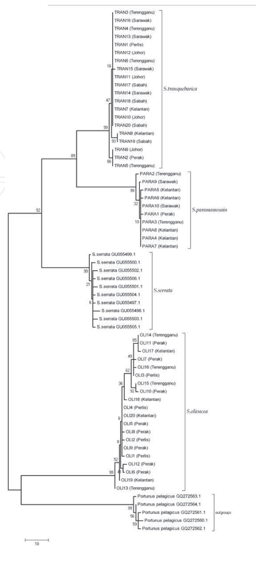
Figure 3. Maximum Parsimony (MP) phylogram showing the relationships among cytochrome c oxidase I (COI) sequences of Scylla species and 5 outgroups of genus Portunus analyzed in the present study. The number at each node represents the bootstrap percentage value based on 1000 replicates and applies the close-neighbour interchange (CNI) using the initial tree by random addition of 100 replicates for the maximum parsimony (MP) analysis generated using MEGA ver. 4.0 [17] software.
