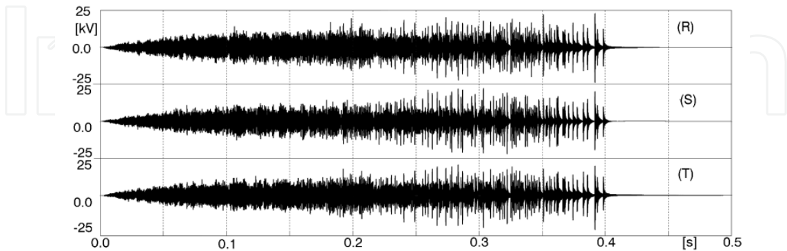
(a) GIS-DS opening
