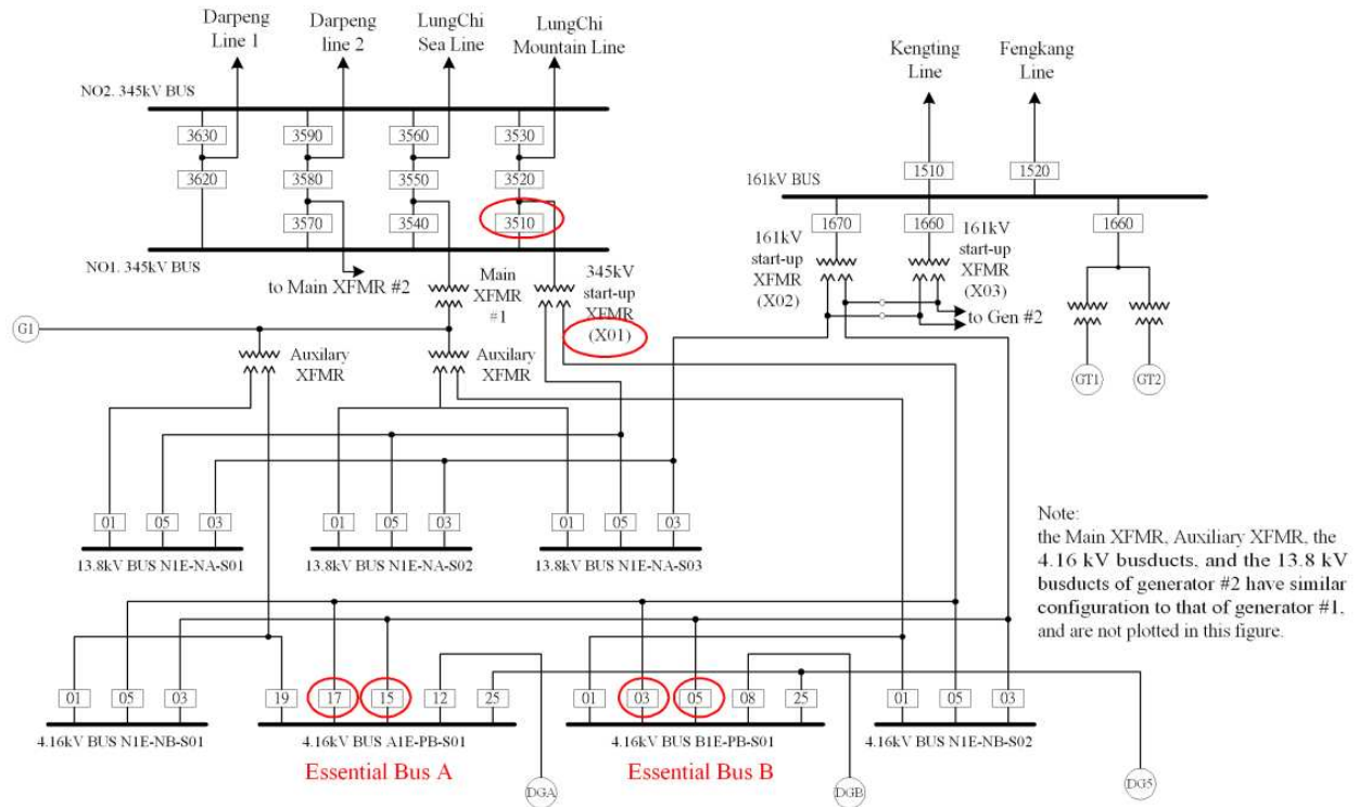
Figure 1. System Configuration of the NPP
