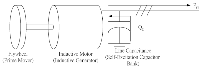
Figure 4. Equivalent Circuit of Motor-Generating Effect.
