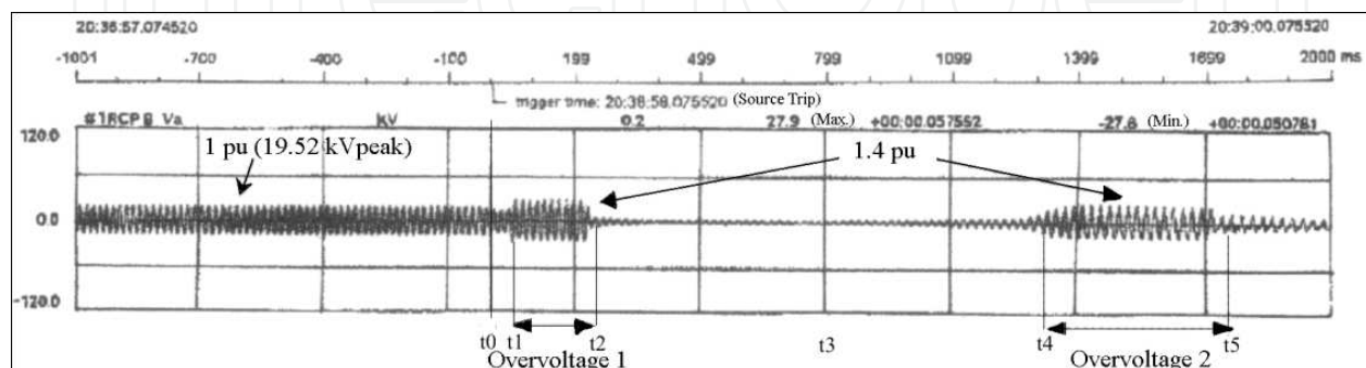
(b) Line-to-Line Voltage Transient Recording of one 13.8 kV motor, Recycle Colling Pump B
