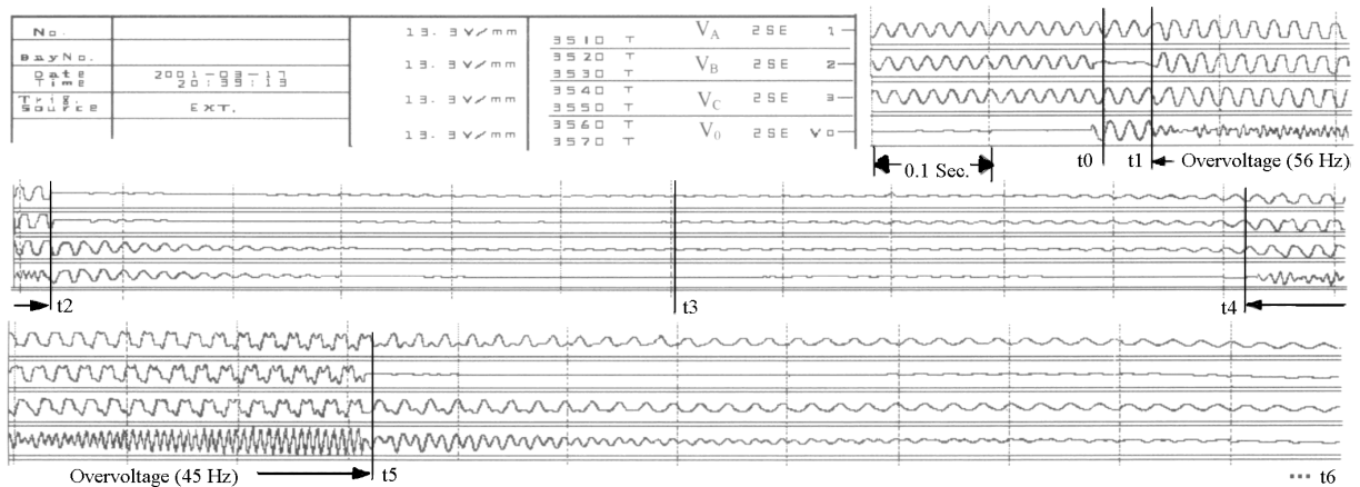
(a) Transient Recording at 345 kV GIS
