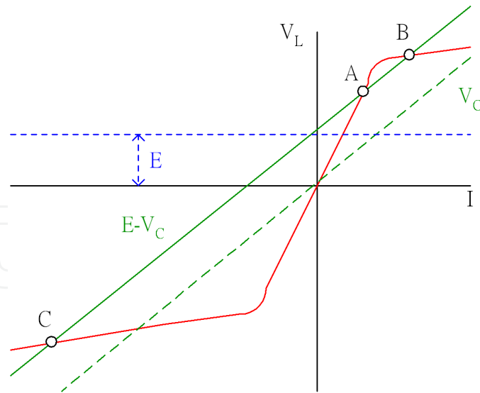
Figure 8. Ferroresonance Phenomenon Explanation
