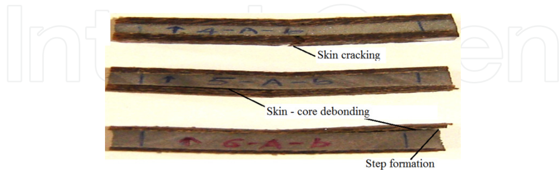
Figure 13. Sandwich failure modes under three point bending loads
