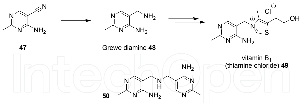
Scheme 15. Production of Grewe diamine for vitamin B 1 .
