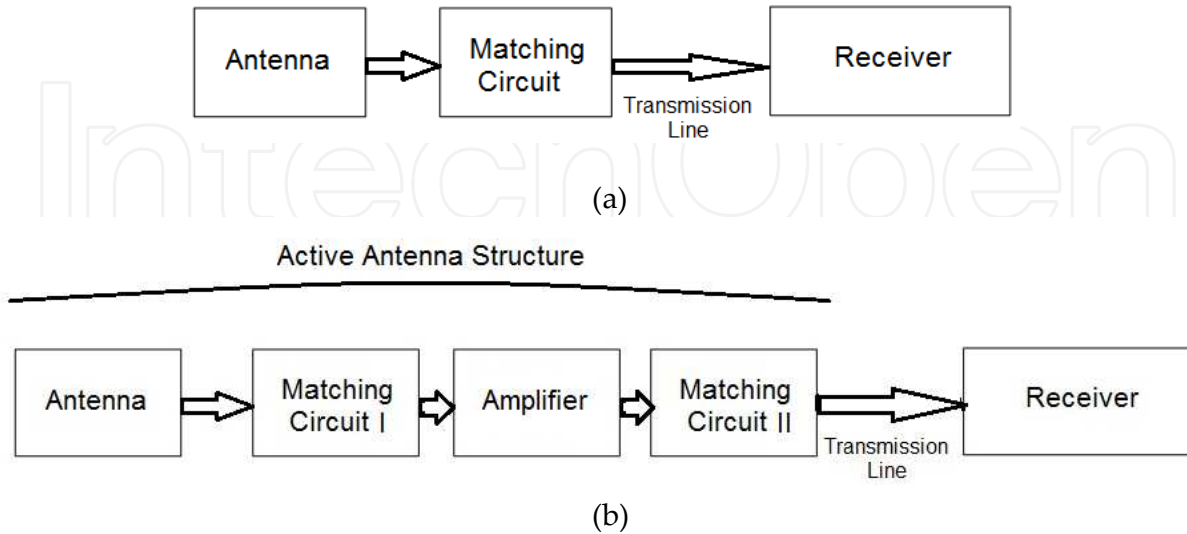
Figure 3. a). Receiving system structure for passive antenna; b). Receiving system structure for active antenna
