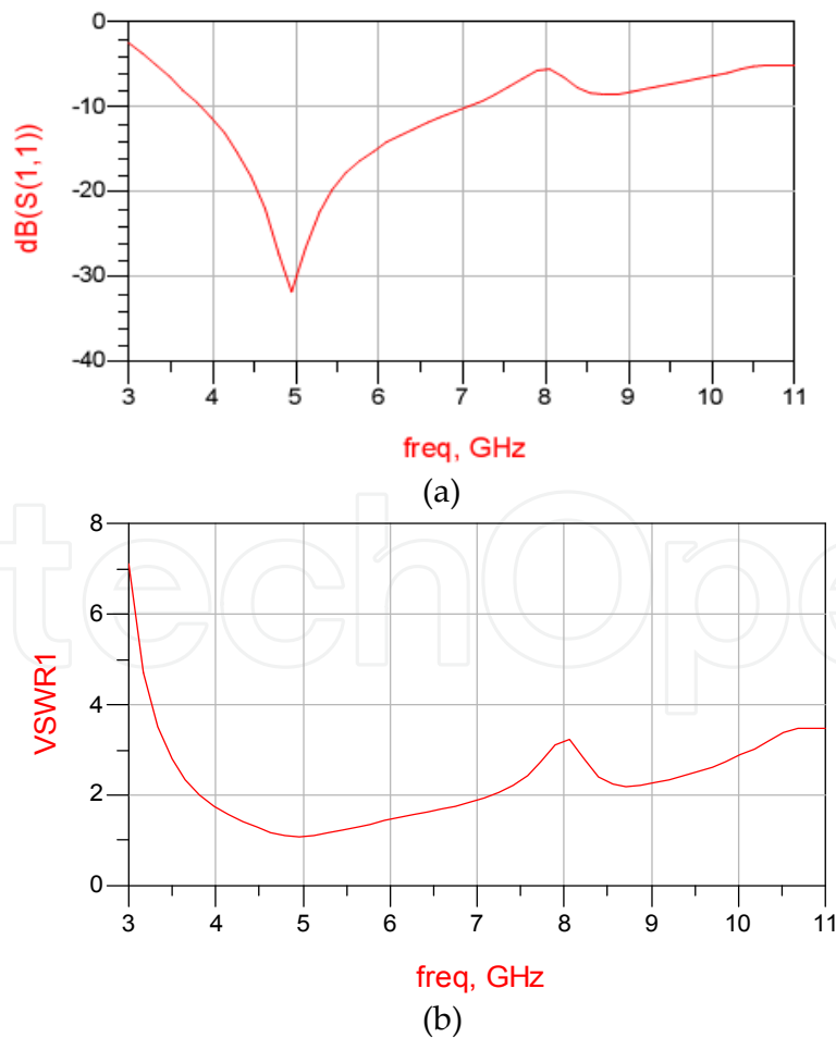
Figure 8. Spiral antenna parameters in the UWB Band; a) S_{11} and b) VSWR
