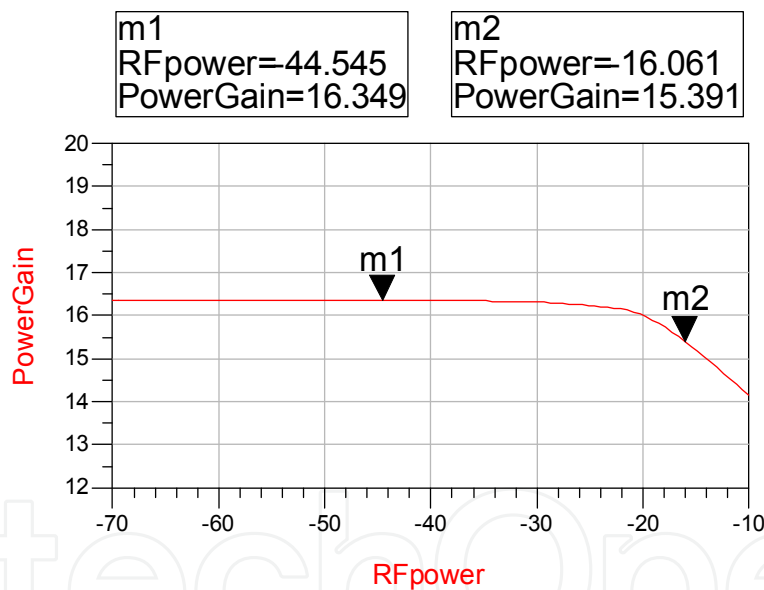
Figure 10. 1dB point calculation in 7GHz. RFpower is input power
