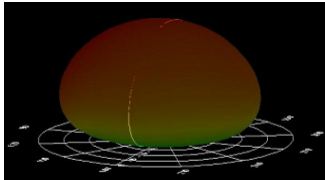
Figure 6. Spiral antenna radiation pattern in 3.36GHz
