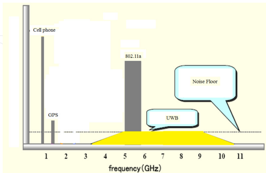
Figure 1. Ultra wideband communications spread transmitting energy
