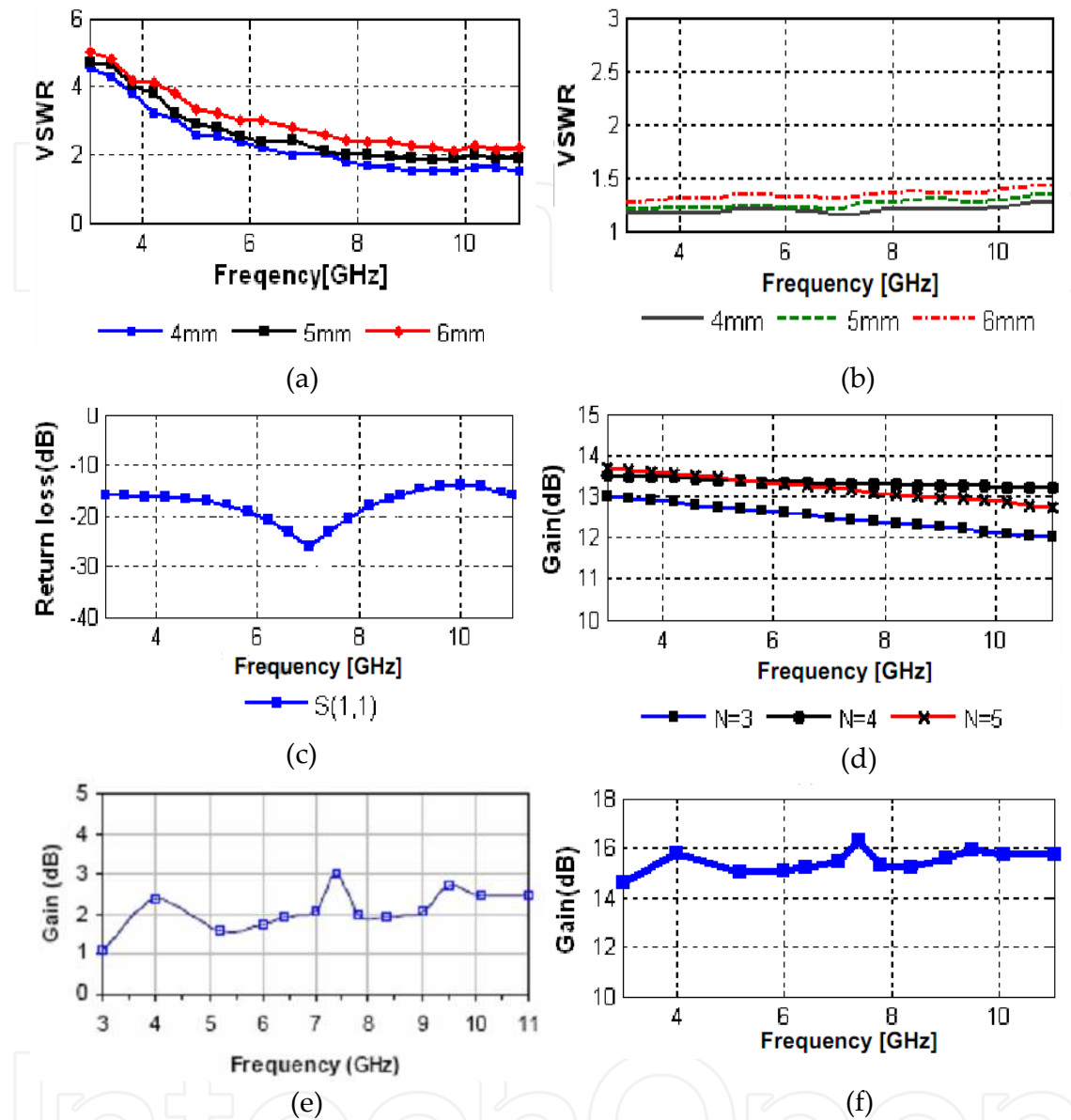
Figure 15. Passive antenna parameters and optimized parameters of active antenna [27]; a) VSWR of passive spiral antenna in w=4, 5 and 6 mm; b) VSWR of optimized active antenna in w=4, 5 and 6 mm; c) Return loss of optimized active antenna; d) Uwb distributed amplifier gain for N=3,4 and 5 ( N is the turns of spiral antenna); e) Gain of passive spiral antenna; f) Gain of optimized active antenna
