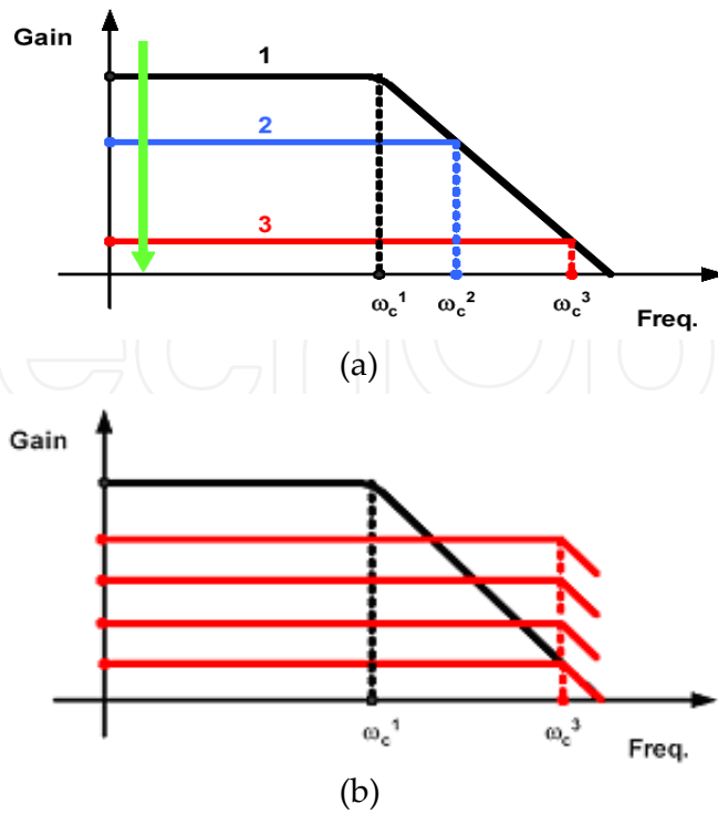
Figure 5. a).Trade-off between gain and bandwidth; b).high gain and wide bandwidth by distributed amplifier
