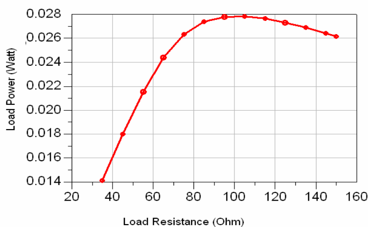
Figure 9. Load power against load resistance
