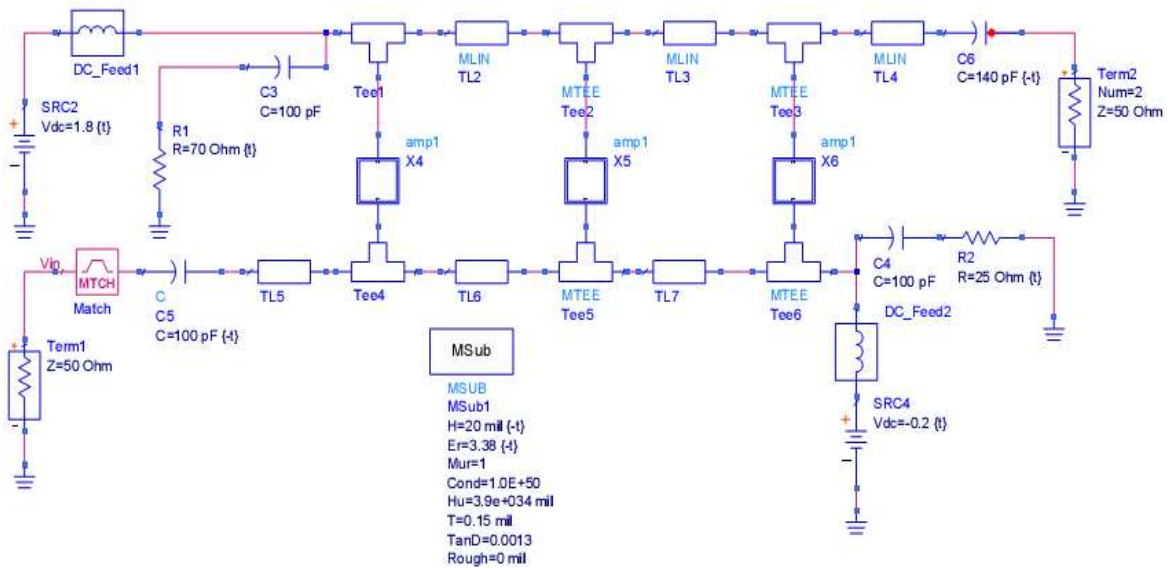
Figure 11. Designed distributed amplifier structure.
