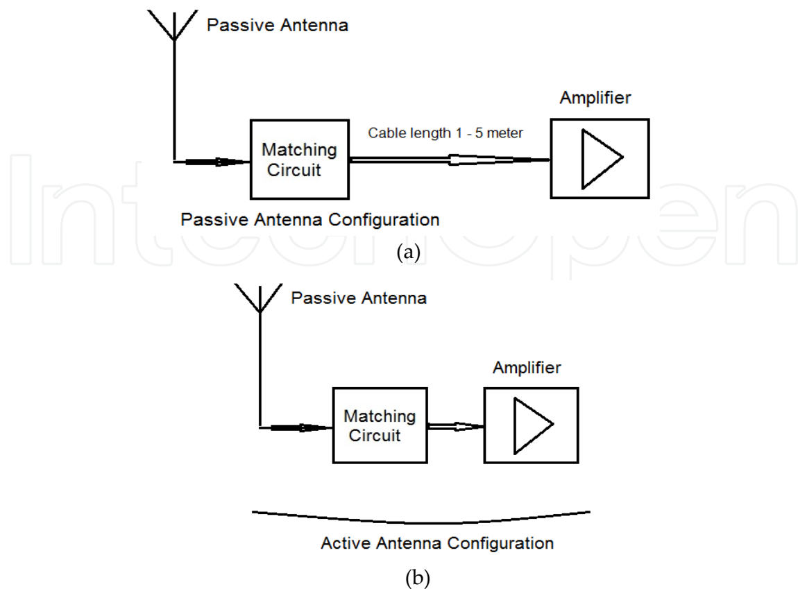
Figure 4. Passive and active antenna assembling comparison
