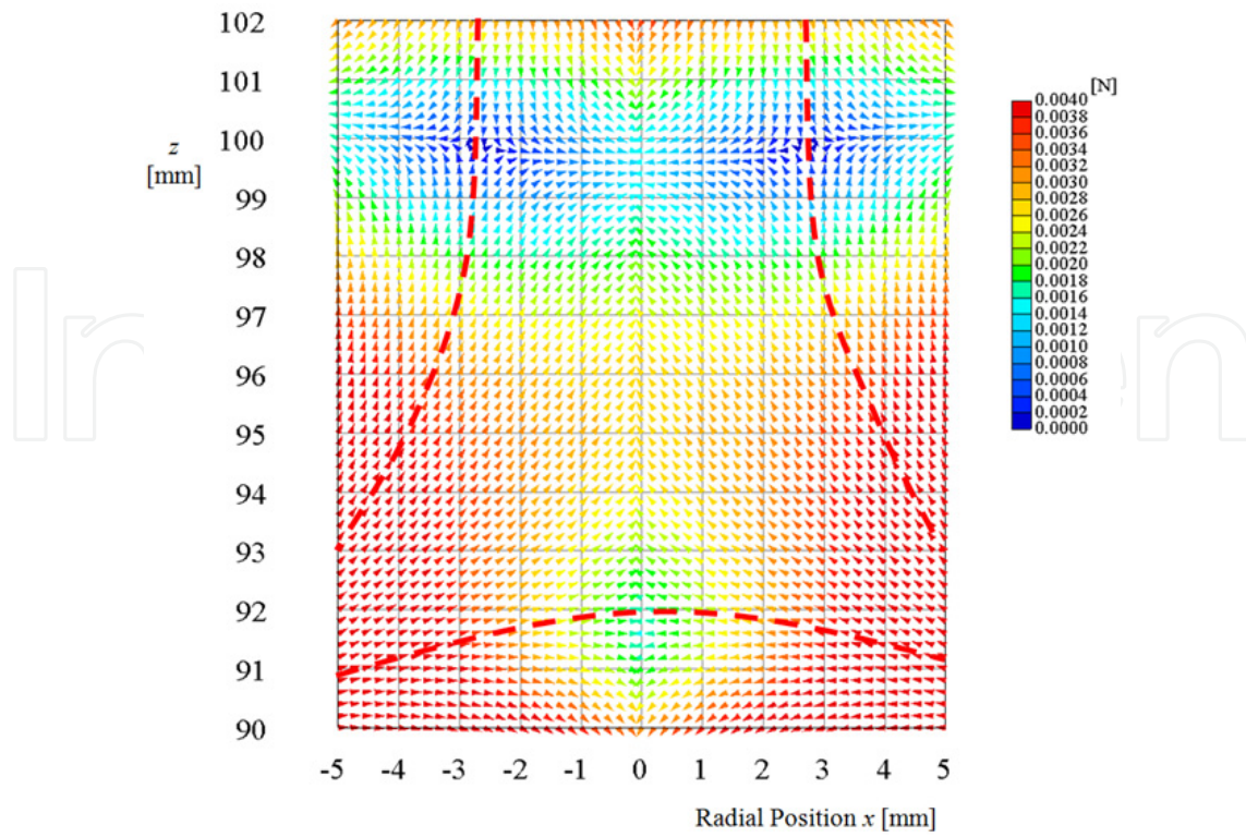
(c) The levitating area when the tilt angle is 0.8^\circ .
