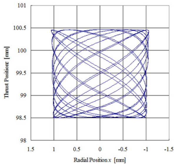
(a) Trajectory of the centre of the rotor magnet.
