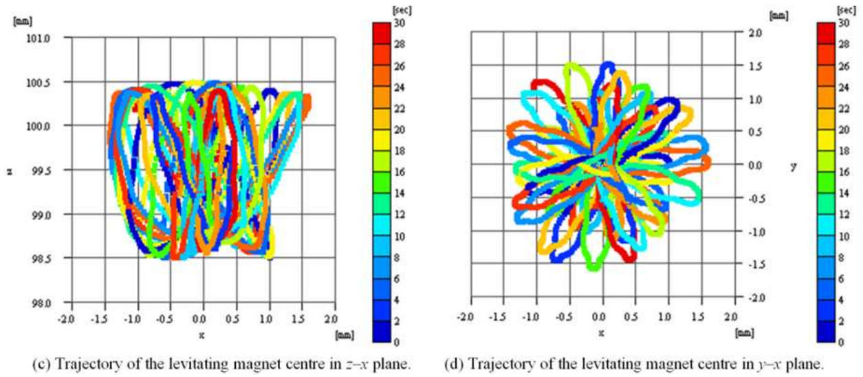
Figure 14. Simulated trajectories of the levitating magnetic top rotating at 1,080 rpm.
