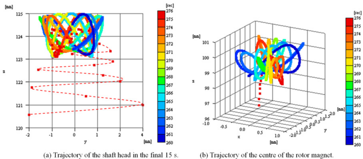
Figure 22. Trajectories of a levitating magnetic top started at 1380 rpm and fall down at 275 s after start.
