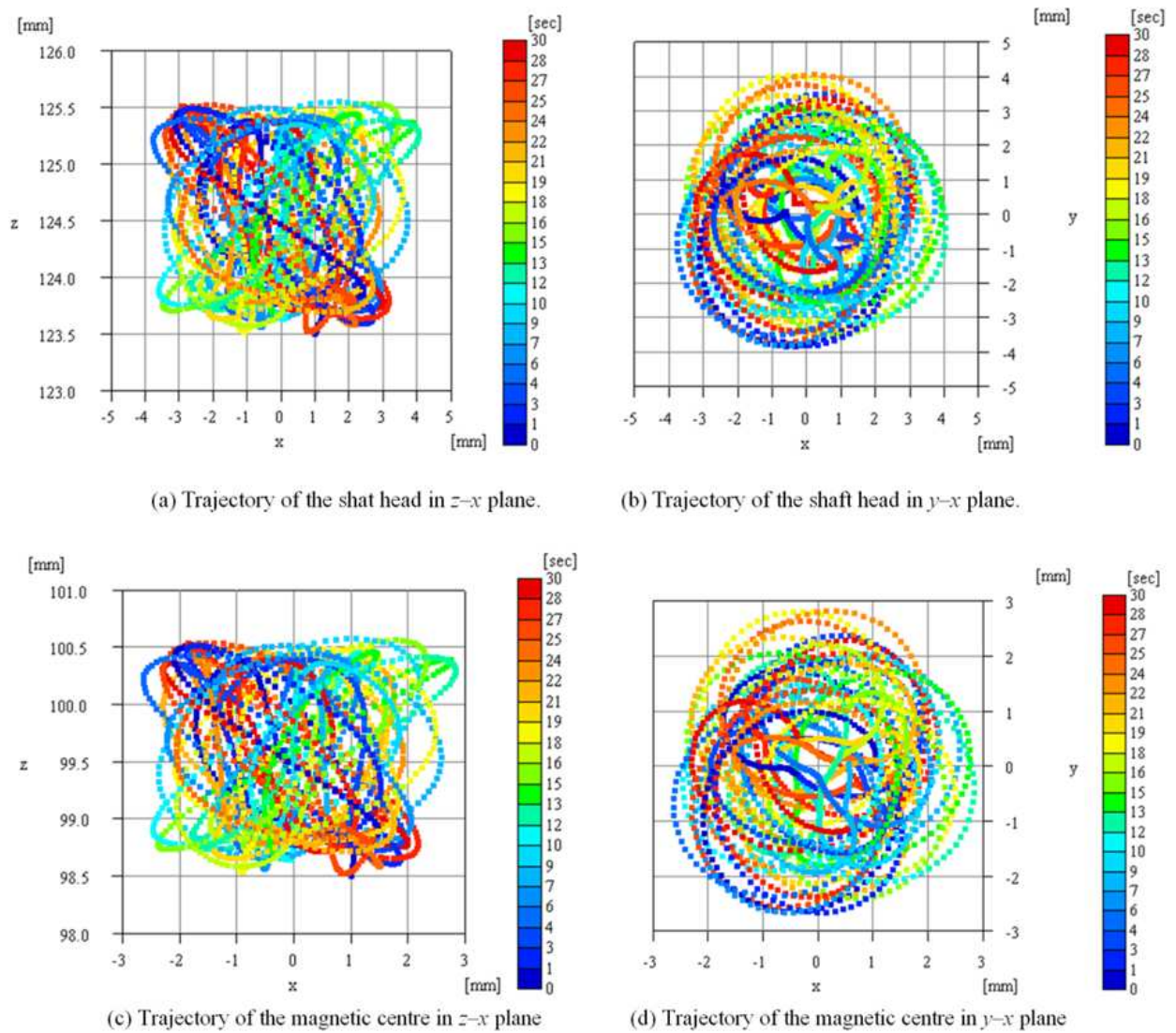
Figure 15. Simulated trajectories of the levitating magnetic top rotating at 3,000 rpm.
