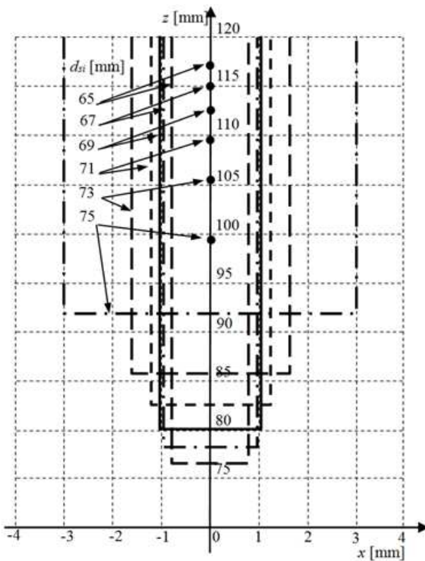
(c) Levitating areas vs. inner diameter of the stator magnet.
