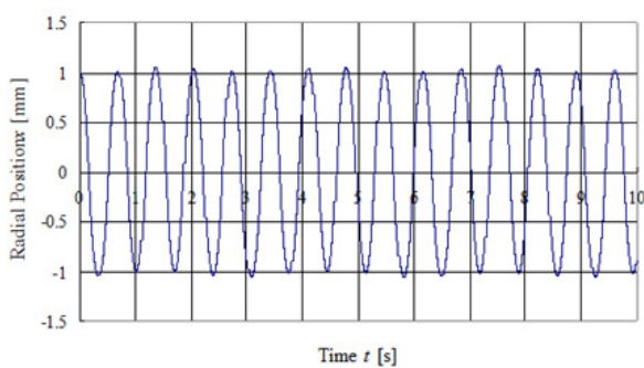
(b) Time dependency of radial motion.
