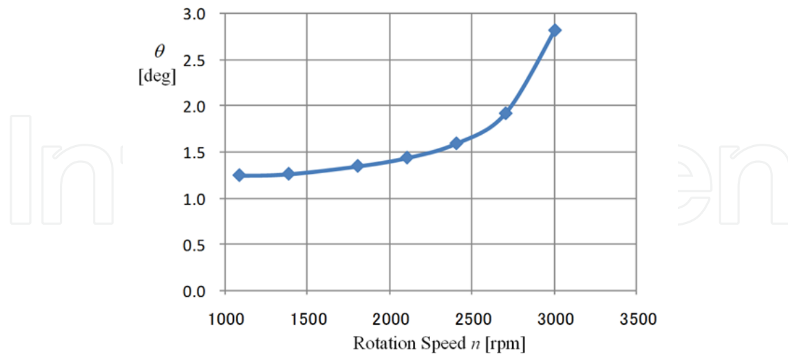
Figure 13. The maximum tilt angle \theta vs. rotating speed.
