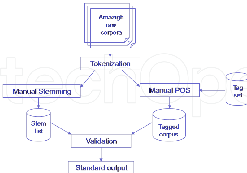
Figure 6. Tagging assistance tool conception.
