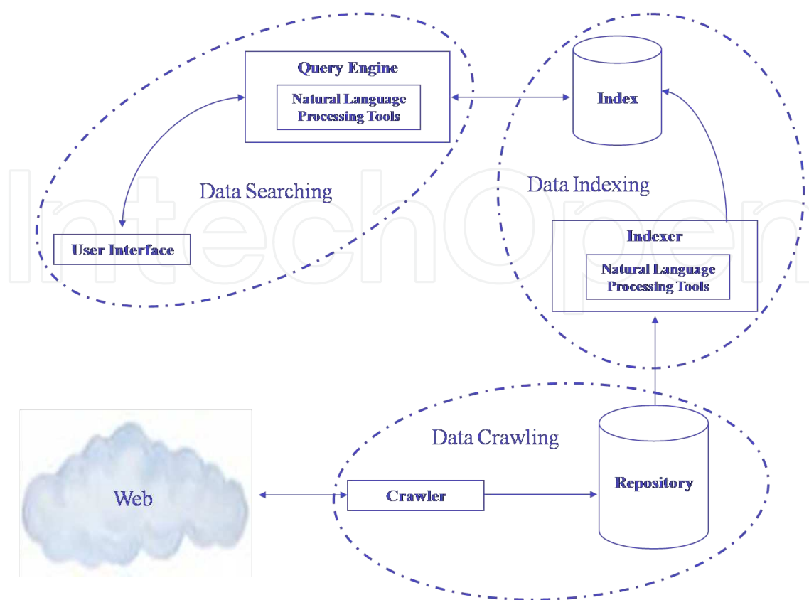
Figure 4. Amazigh search engine architecture.
