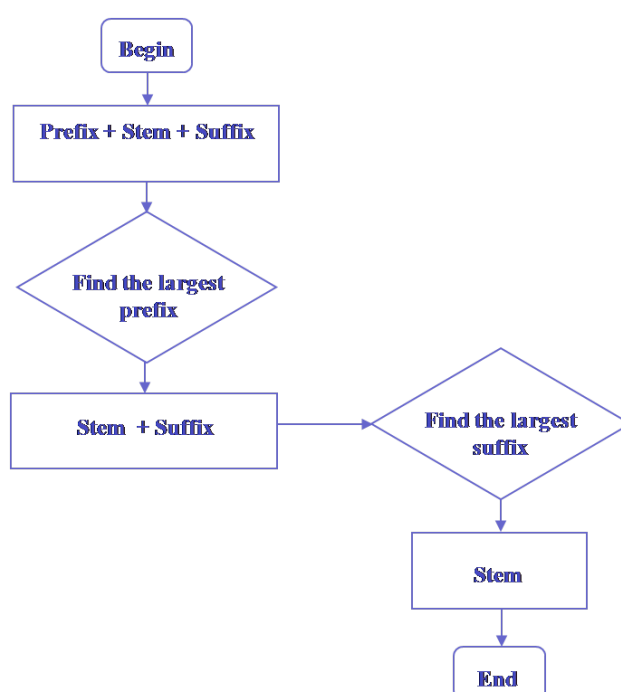
Figure 3. Amazigh light stemming process.
