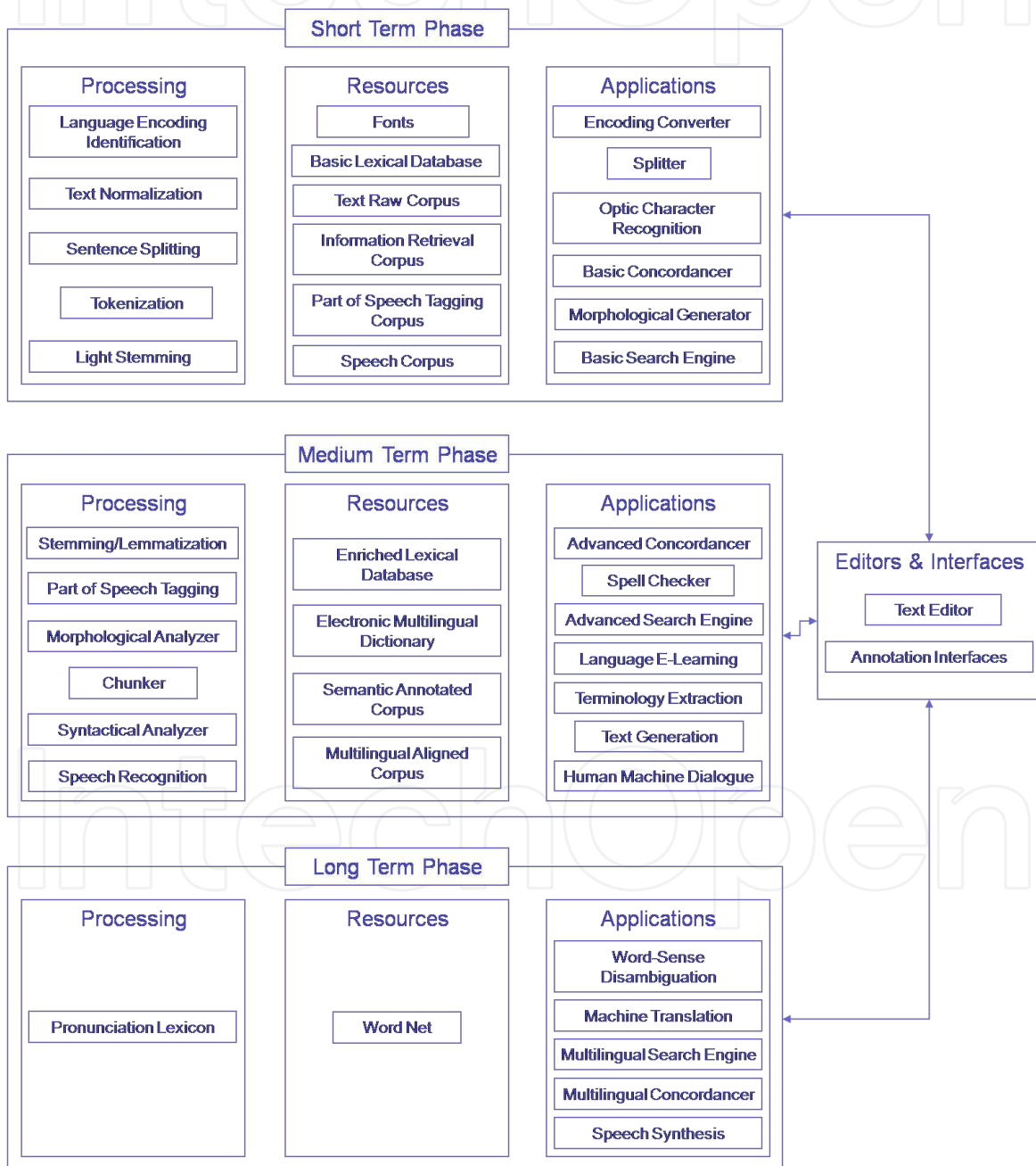
Figure 1. Road map for under and less resourced languages.
