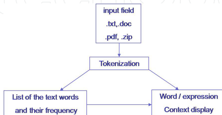
Figure 5. Amazigh concordancer conception.
