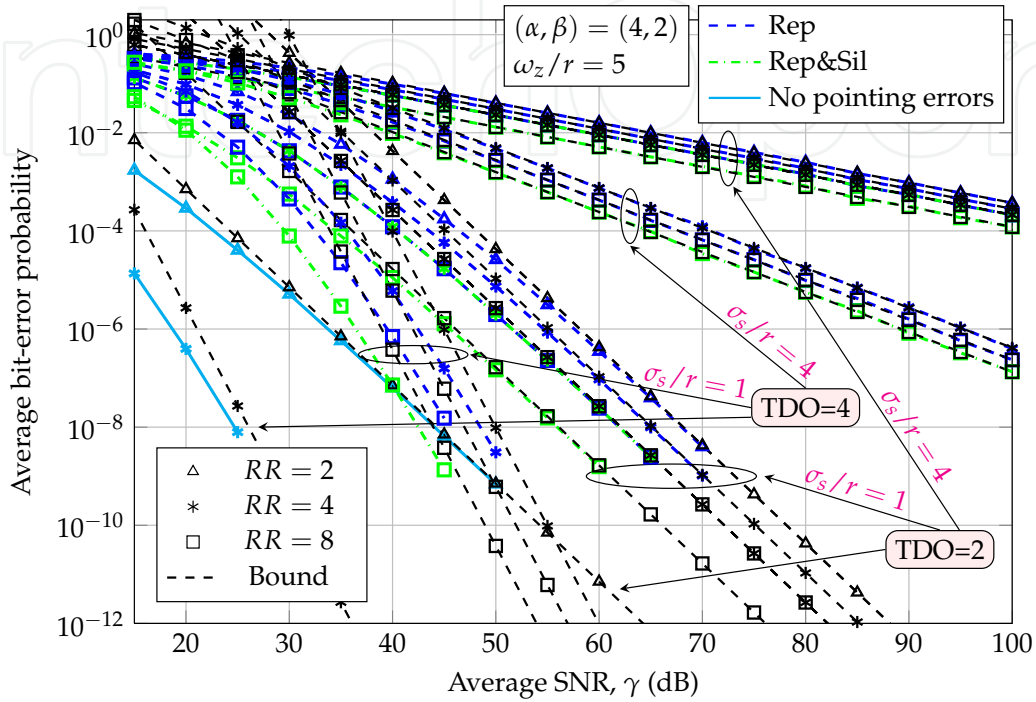
Figure 3. BER performance in FSO IM/DD links using different rate-adaptive transmission schemes over gamma-gamma atmospheric channels with/without pointing errors, assuming TDO= {2, 4} and values of normalized jitter of \sigma_s/r = \{1, 4\} and normalized beamwidth of \omega_z/r = 5 .
