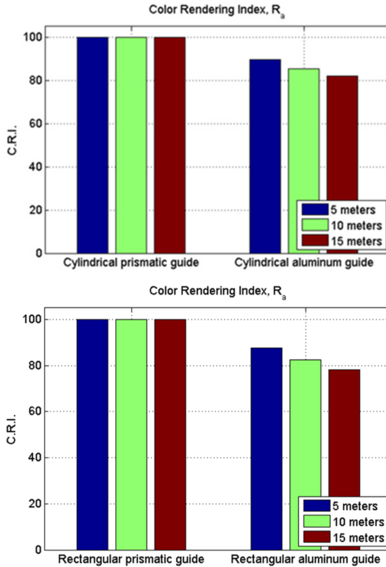
Figure 13. CRI of measured lightguides (cylindrical and rectangular).
