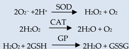
Figure 2. The chemical reactions involving ROS and antioxidant enzymes.
