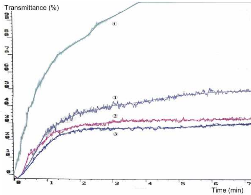
Figure 7. ADP-initiated irreversible aggregation of platelets in the presence of aptotinin, SBTI and trypsin in vitro. The platelet aggregation was initiated by the addition of the 25 mkM ADP. 1 – controle; 2 – aprotinin - 1%; 3 – SBTI - 1%; 4 – trypsin – 0,1%.
