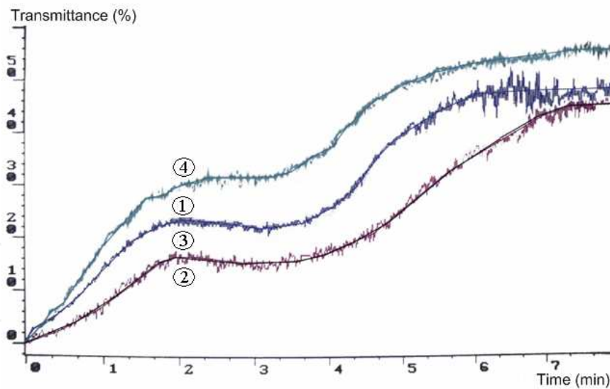
Figure 8. Adrenalin-initiated two-phase aggregation of platelets in the presence of trypsin, aptotinin and SBTI in vitro. The platelet aggregation was initiated by the addition of the 25 mkM adrenalin. 1 – controle; 2 – trypsin - 0,1%; 3 – aprotinin - 1%; 4 – SBTI - 1%.
