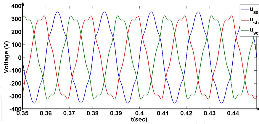
Figure 7. Distorted-unbalanced grid voltages
