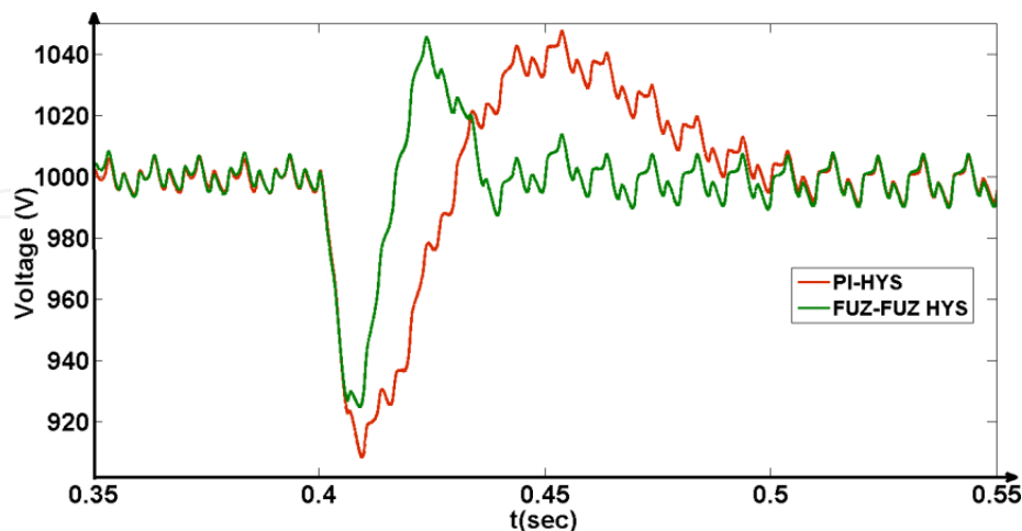
Figure 13. Dc bus voltage response, for both control schemes
