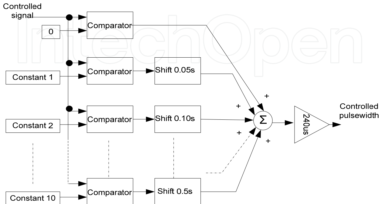
Figure 5. Signal comparator and shifting technique
