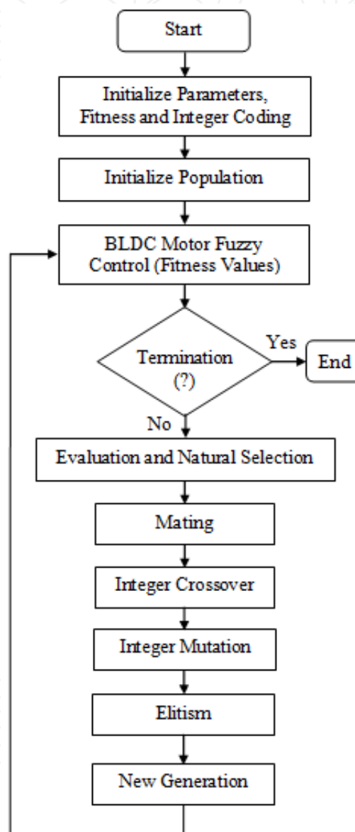
Figure 4. Flowchart of the Real Coded GA based fuzzy controller
