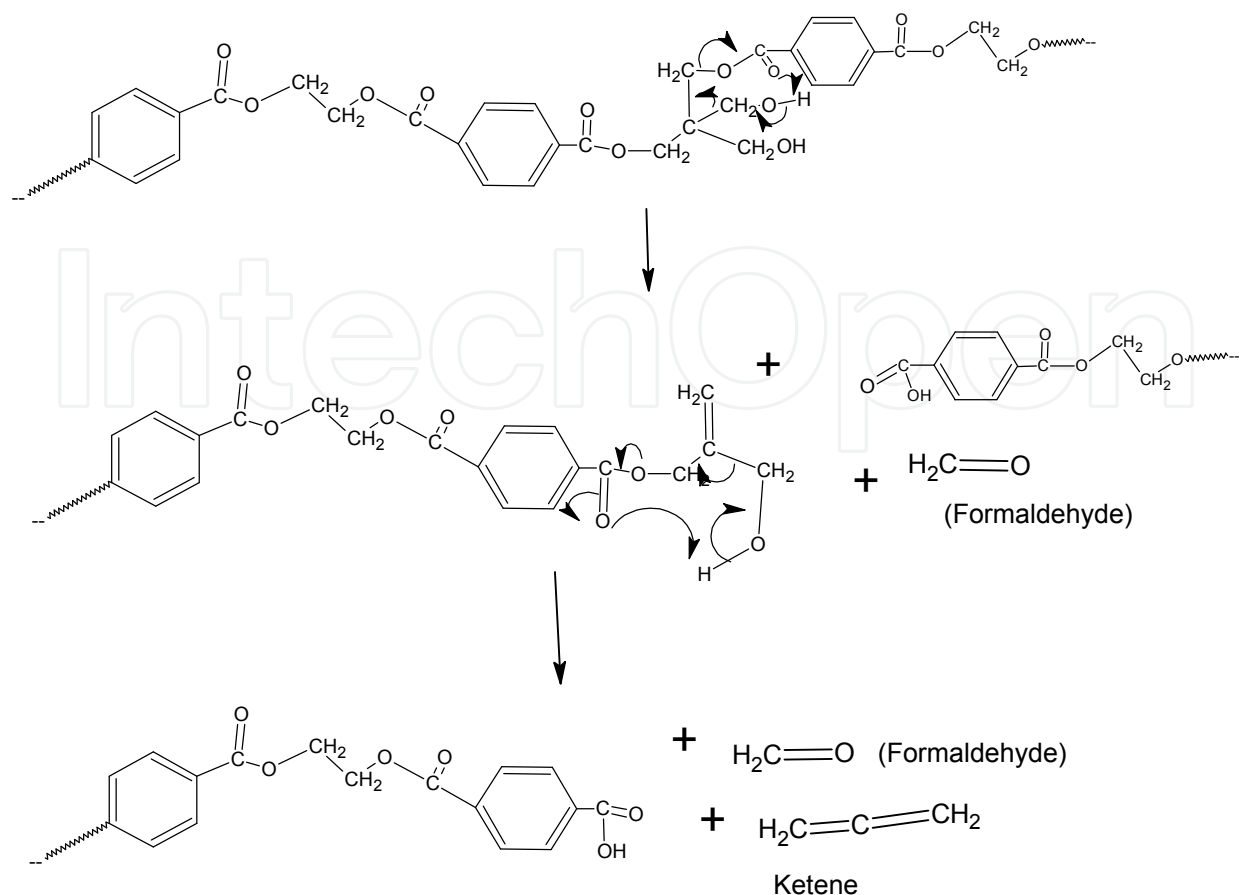
Scheme 12. Mechanism of Degradation in polyester containing penta erithritol moieties
