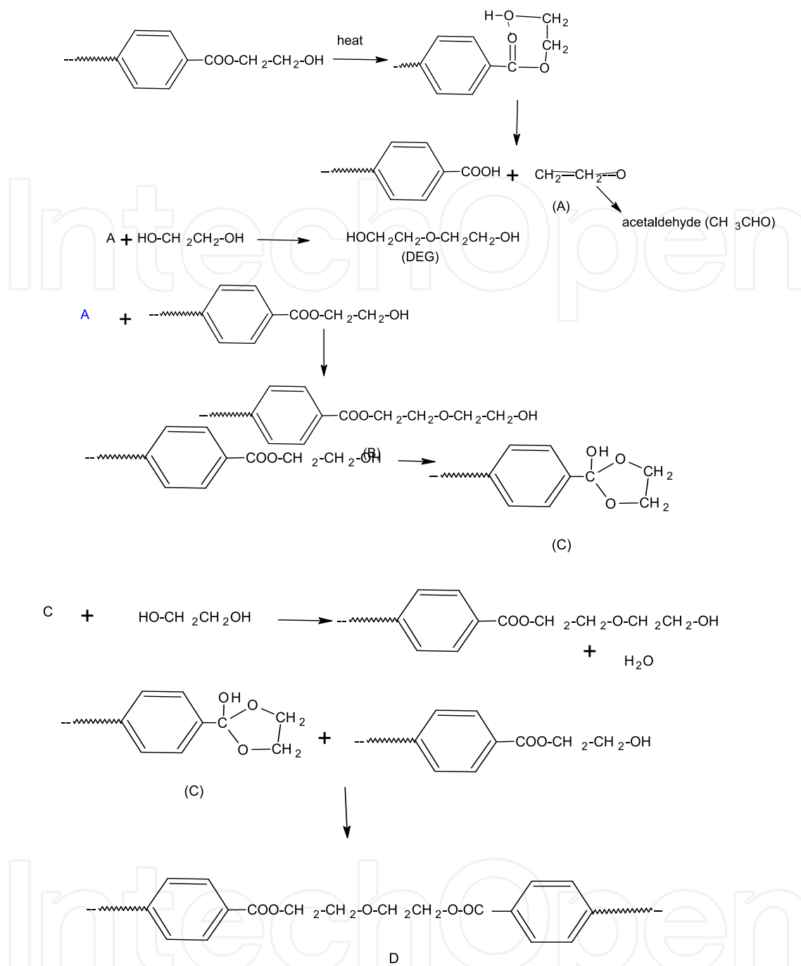
Scheme 10. Mechanism of DEG formation
