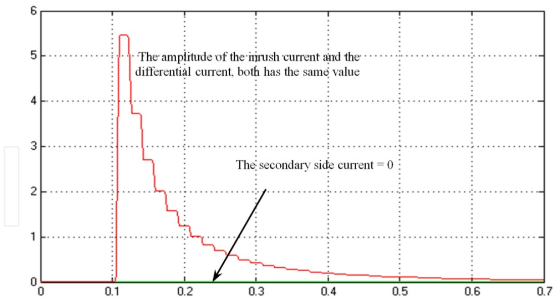
Figure 15. Amplitude comparator results for the 1 st case.
