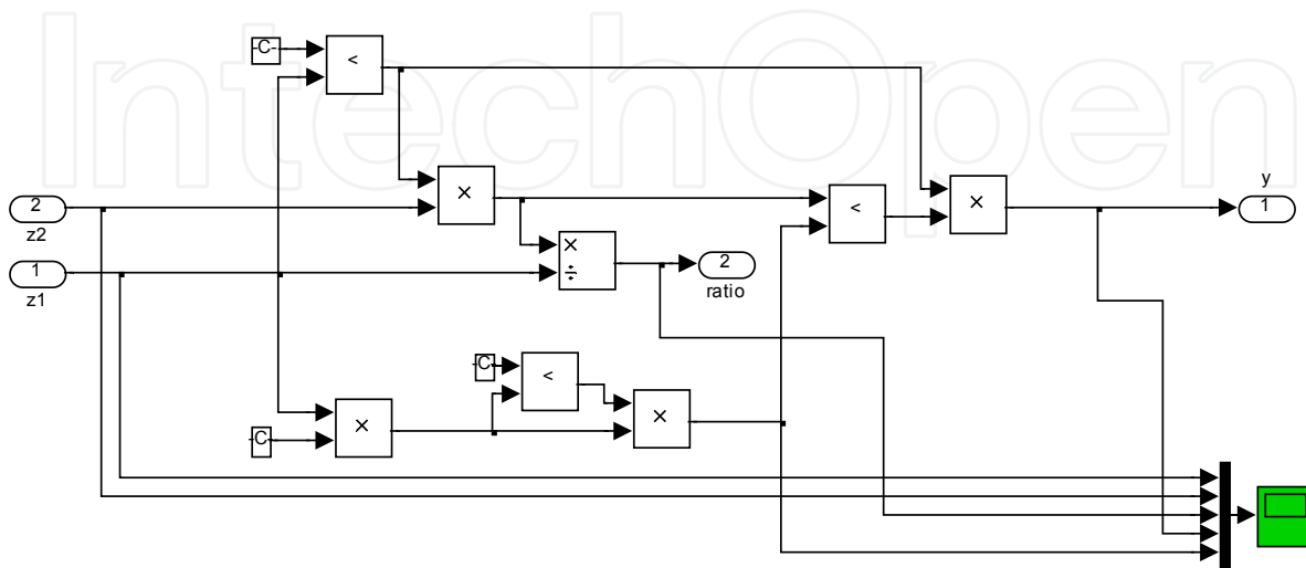
Figure 12. The ratio block contents
