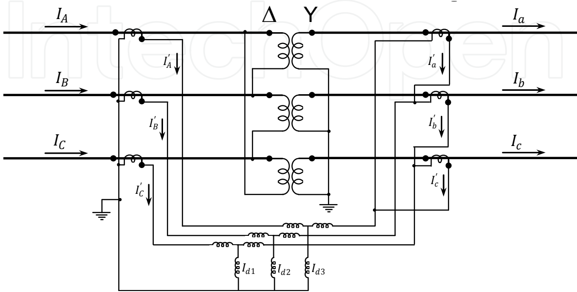
Figure 4. Connection of differential protection of 3-phase Δ-Y transformer
