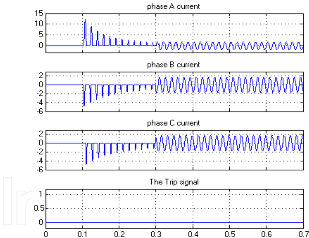
Figure 16. Normal load current starts flowing at 0.3sec.
