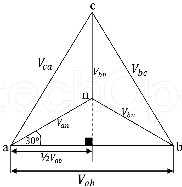
Figure 5. The relationship between line to line voltage and the phase to neutral voltage and the phase shift between them which reflects the phase shift in Y-Δ or Δ-Y connected transformers
