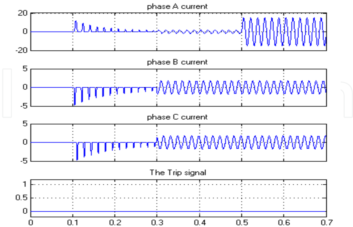
Figure 23. Increase of phase A current due to the occurrence of the fault at 0.5 sec for loaded transformer
