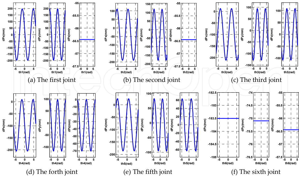
Figure 12. The relation between angle of joints and the end effector differential translation
