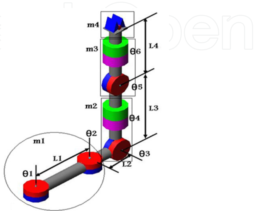
Figure 6. The geometrical model of surgical manipulator
