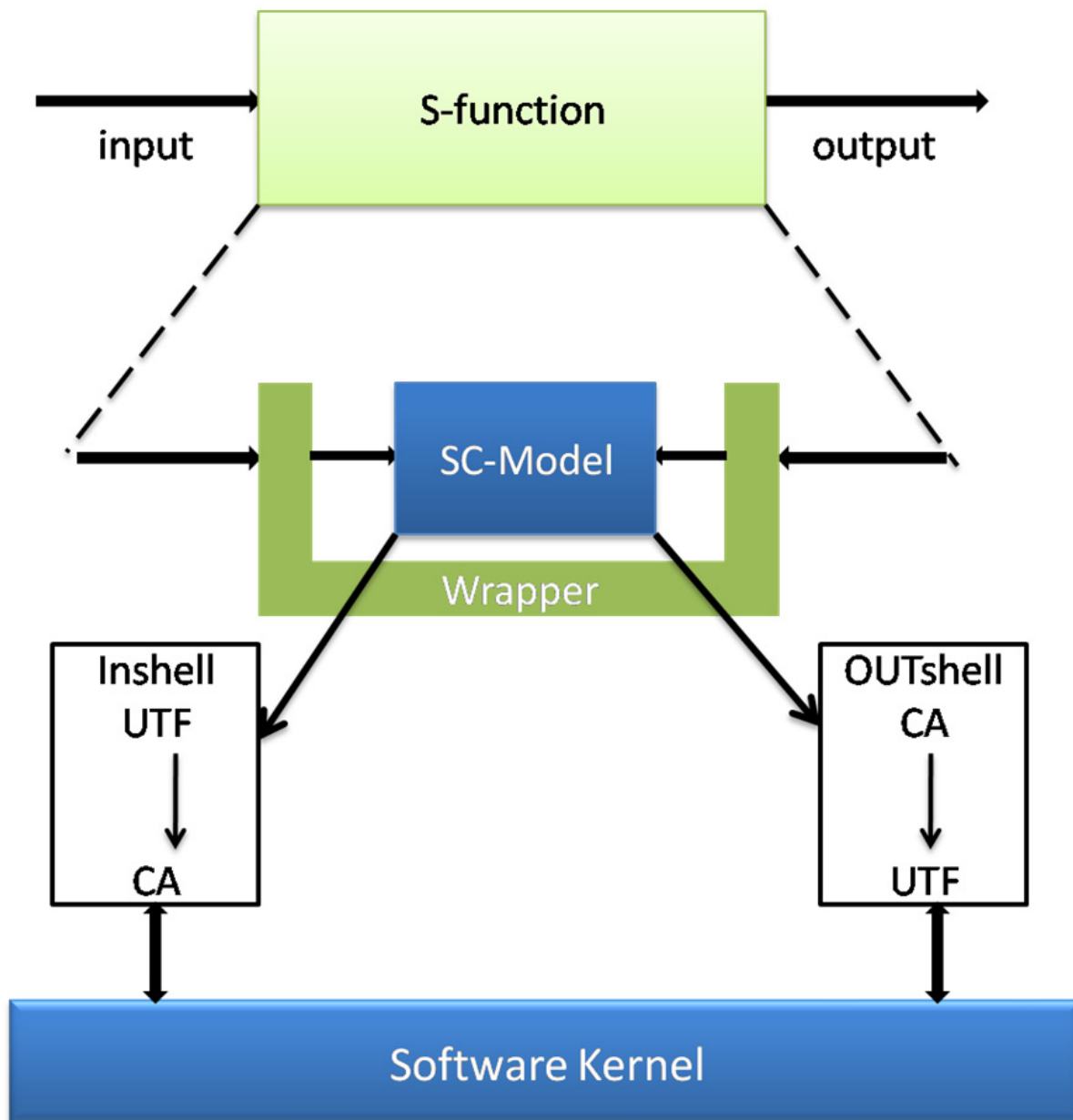
Figure 1. Integrated SystemC in Simulink S-Function.
