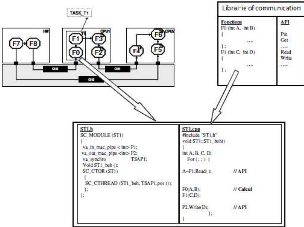
Figure 5. Generating a task from a set of blocks in Simulink.
