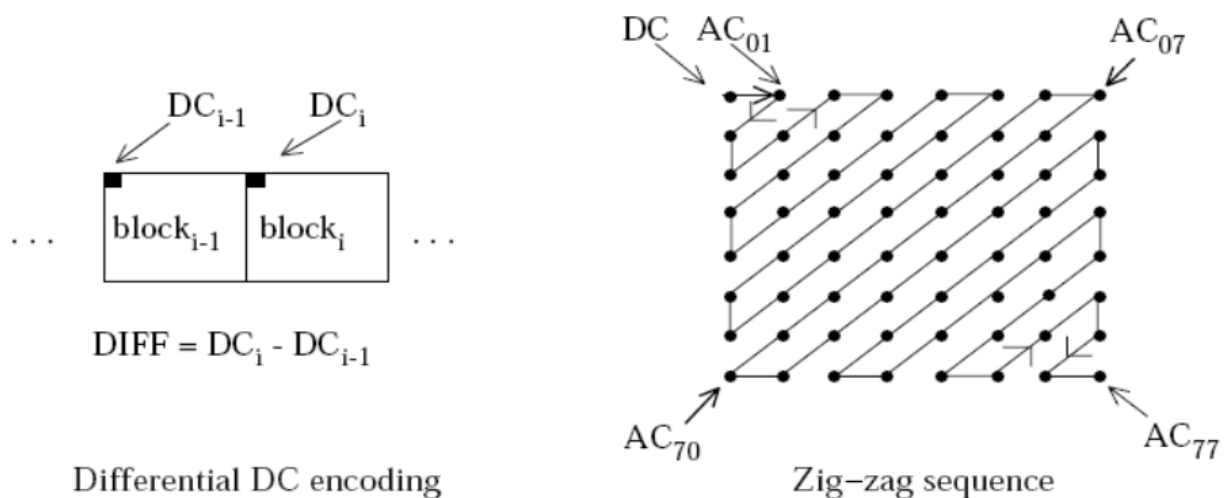
Figure 7. Preparation of Quantized Coefficients for Entropy Coding
