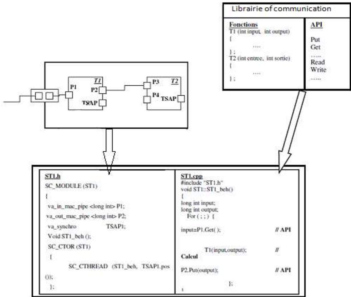
Figure 4. Generating a task from a basic block.
