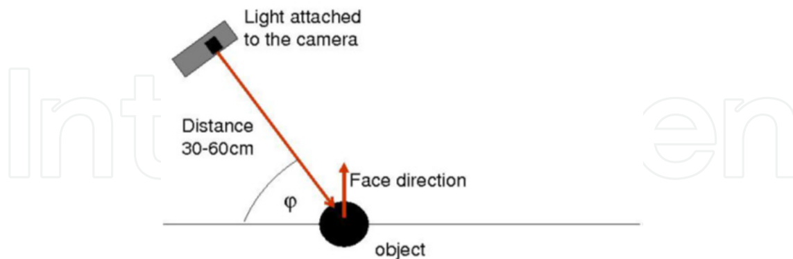
Figure 30. View from above camera configuration
