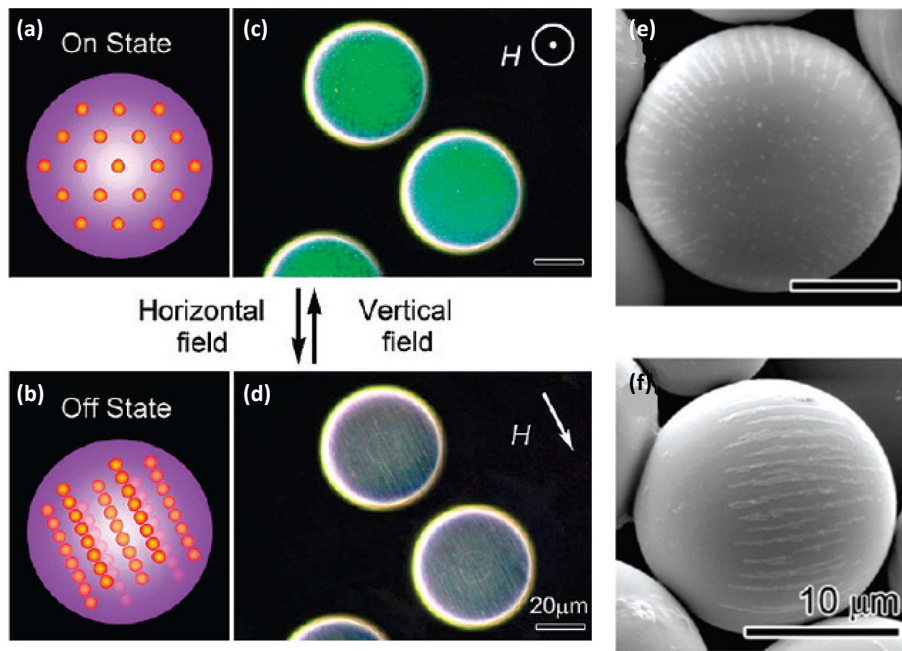
Figure 9. (Color online) Magnetochromatic microspheres switched between ‘on’ and ‘off’ states by rotating external fields [84, 85]. Schematic illustrations, optical images, and the corresponding SEM photographs of ‘on’ and ‘off’ states are (a), (c), (e), and (b), (d), (f), respectively.
