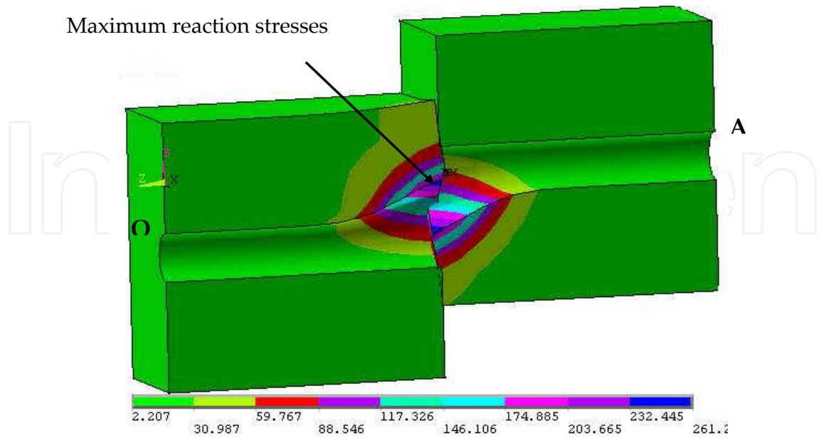
Figure 27. Yield stress induced in 20 MPa concrete without pre-tension condition
