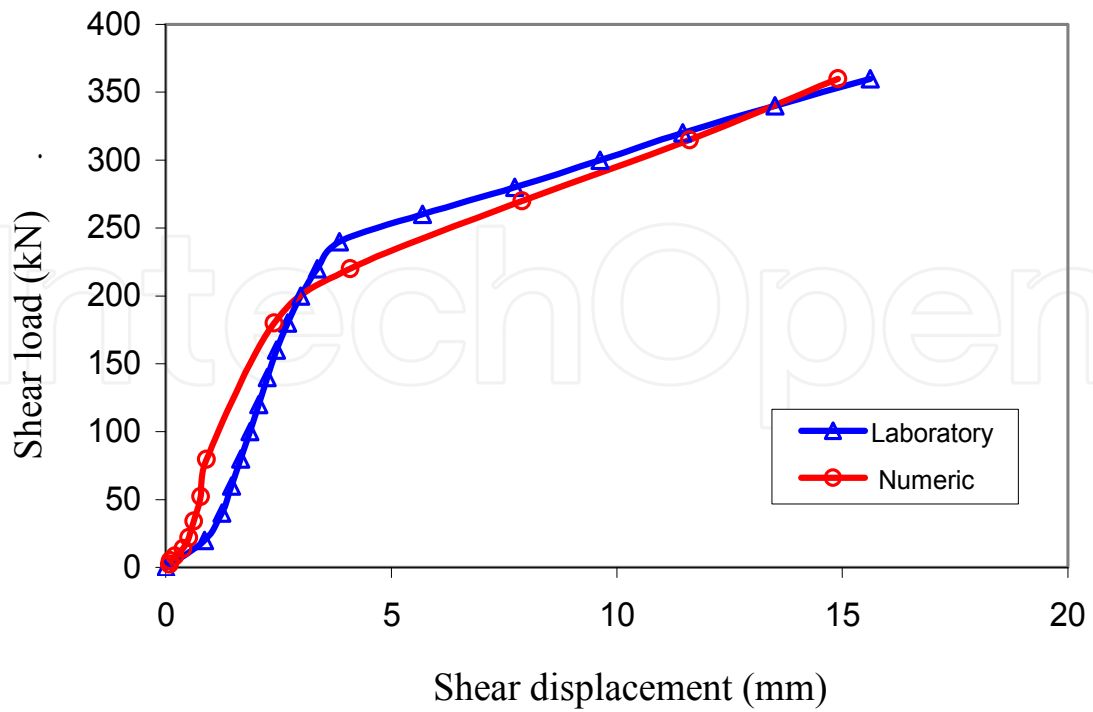
Figure 10. Load-deflection in 80 kN pretension bolt load and 40 MPa concrete
