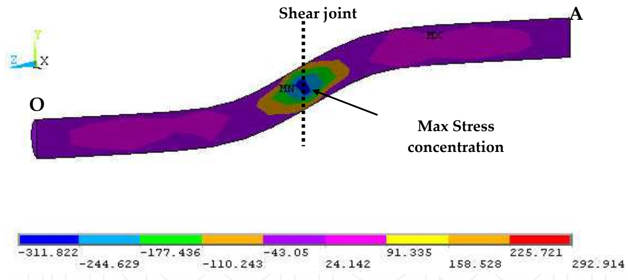
Figure 18. Shear stress contour in the concrete 20 MPa without pre-tension
