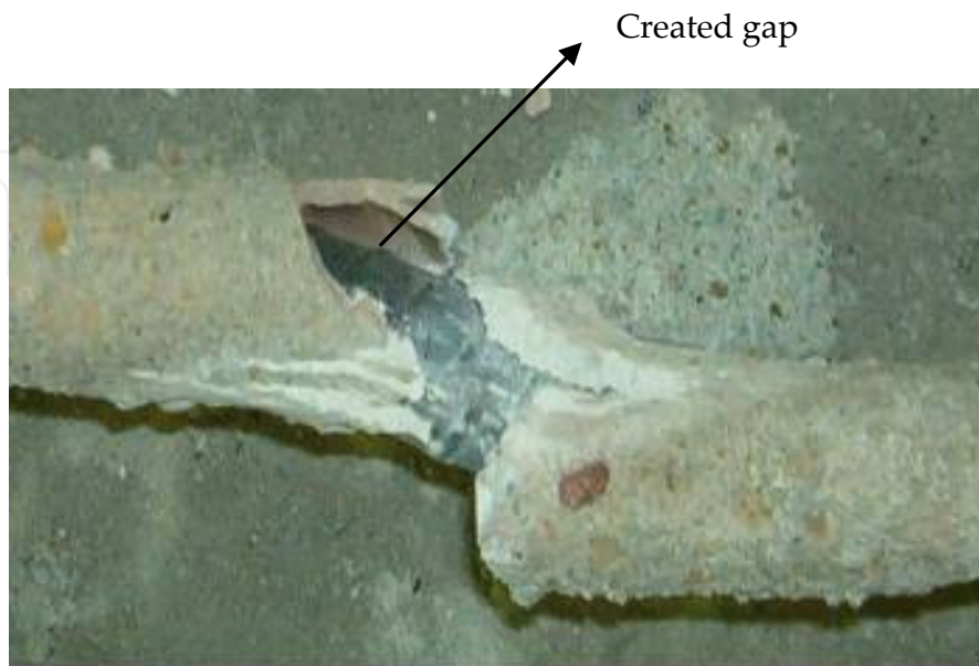
Figure 34. Gap formation in post failure region in 20 MPa concrete in the laboratory test
