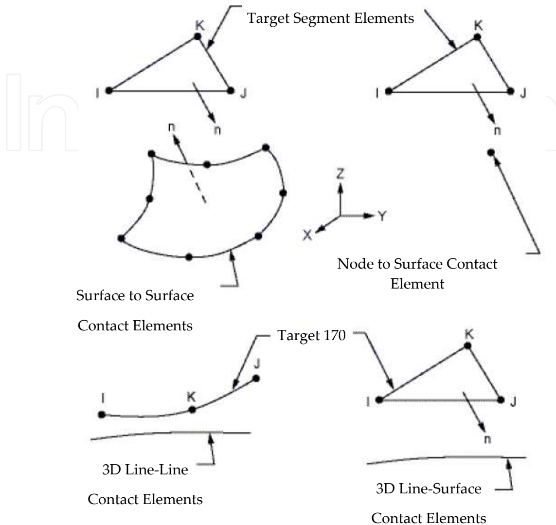
Figure 8. Target 170 geometry (Ansys 2012)
