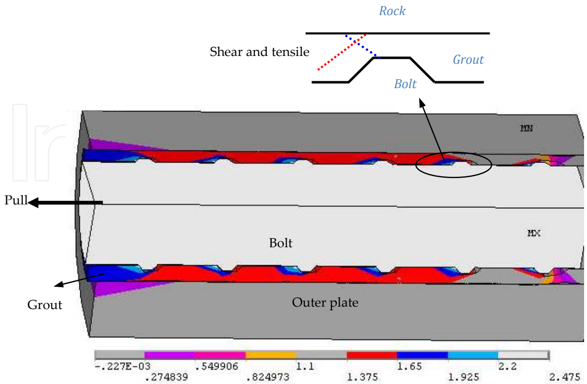
Figure 37. The bolt movement in pulling test
