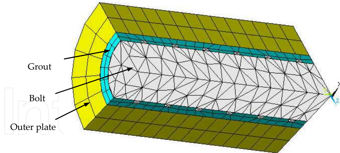
Figure 36. FE mesh: a quarter of the model
