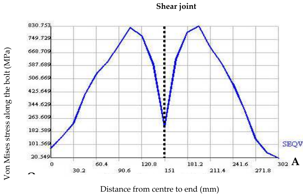
Figure 17. Von Mises stress trend in 20 MPa concrete without pre-tension
