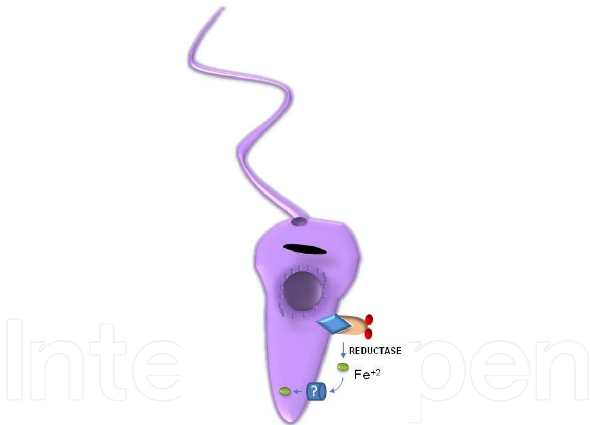
Figure 5. Iron uptake from Transferrin by Leishmania chagasi promastigotes. A non-specific receptor, Lc Tbp \blacklozenge , binds TF \blacktriangledown , allowing a parasite-associated or secreted reductase to reduce the ferric iron \bullet from holoTF, and in this way, the TF affinity for iron diminishes, allowing ferrous iron \bullet to be internalized by the parasite.
