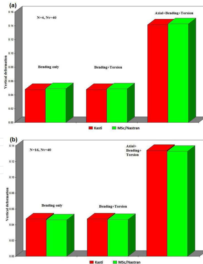
Figure 4. Vertical deformations of armchair carbon nanotubes with lattice translational indices of 4 and 16, respectively. Three cases are considered: 1) bending stiffness only, 2) bending + torsion and 3) axial+bending+torsional.
