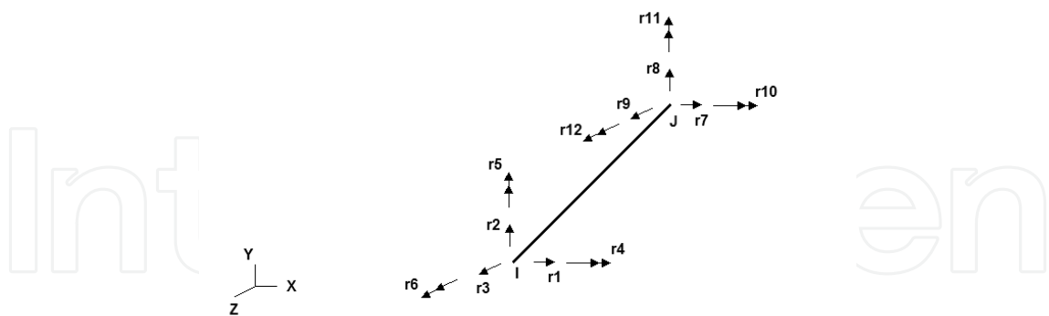
Figure 2. Space frame element.
