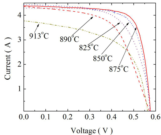
Figure 8. Comparison of the illuminated current-voltage (LIV) characteristics of the cells fabricated with local back contact through the opening in SiNx film on rear surface by varying the peak temperature of the co-firing profile, as indicated with the traces.
