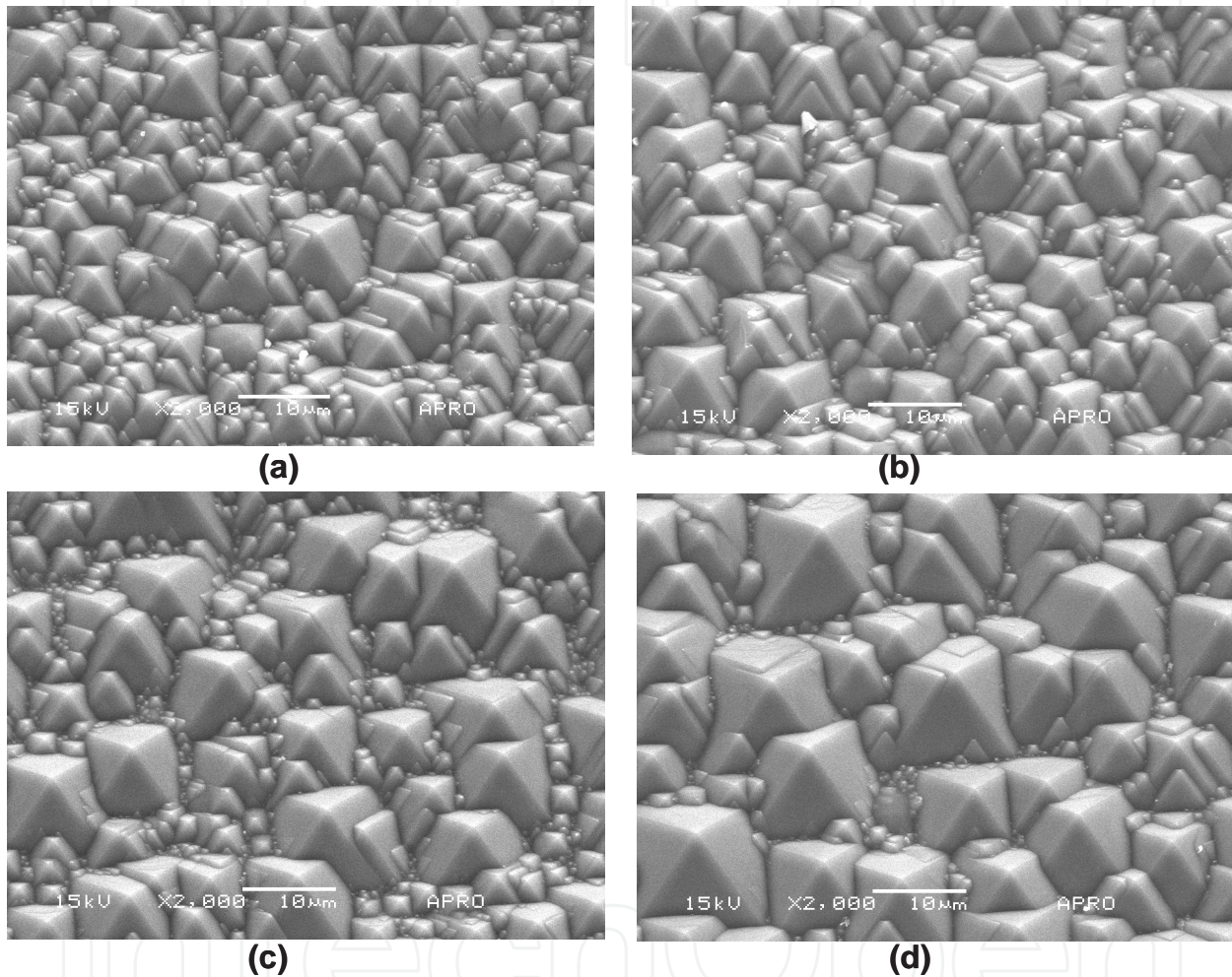
Figure 4. SEM micrographs of the silicon surface textured for (a) 25 min, (b) 30 min, (c) 35 min, and (d) 40 min in and solution containing NaOH ( 2 wt. %) in DI-W water and IPA ( 6 wt. %) at 82^{\circ}\text{C} .
