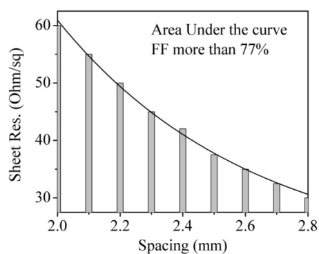
Figure 7. The relation between the sheet resistance with finger spacing for the available range of more than 77% of the fill factor.
