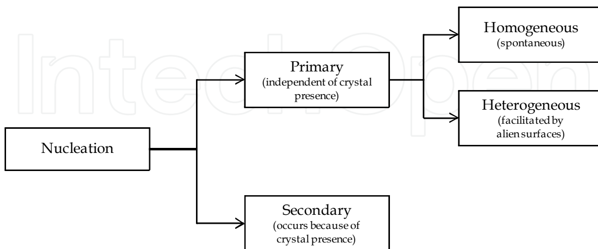
Fig. 1. Mechanisms of nucleation
