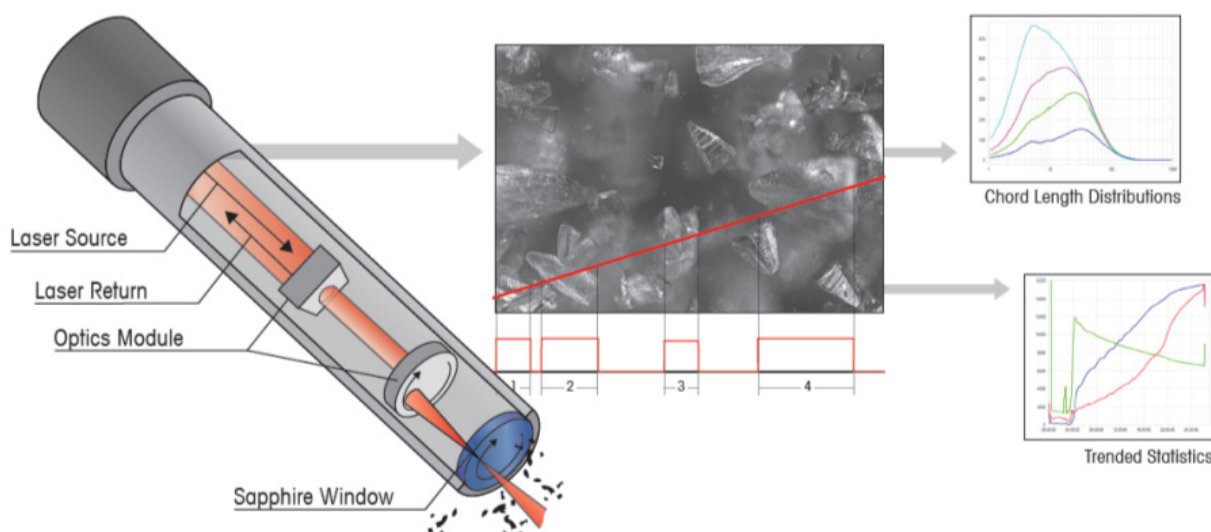
Fig. 2. Measurement principles of the Lasentec FBRM probe.
