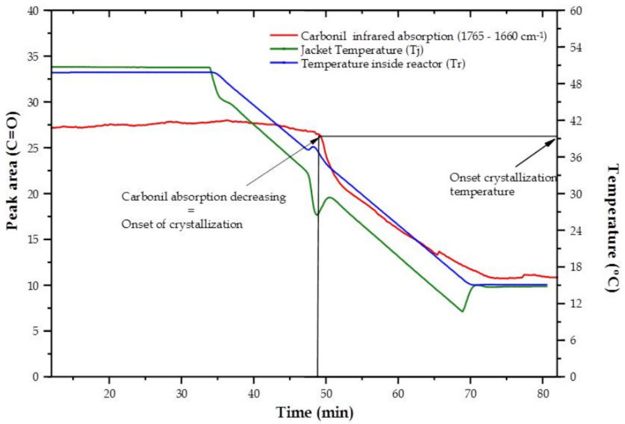
Fig. 13. Absorption curve of the carbonyl C=O ( 1765\text{-}1660\text{ cm}^{-1} ) in ethanol, the temperature inside the reactor ( T_r ) and jacket temperature ( T_j ), obtained from crystallization experiments using an ethanol solution with initial concentration of 22% , cooled at a rate of 1^\circ\text{C}/\text{min} and stirring rate of 300 rpm.
