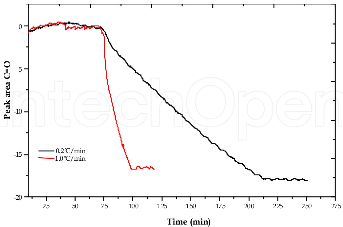
Fig. 14. Infrared absorption curve of the carbonyl C=O ( 1765\text{-}1660\text{ cm}^{-1} ) of adipic acid during crystallizations performed at cooling rates of 1.0 and 0.2^\circ\text{C}/\text{min} .
