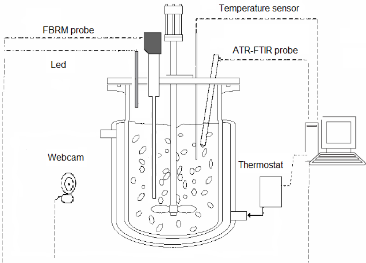
Fig. 4. Experimental setup.
