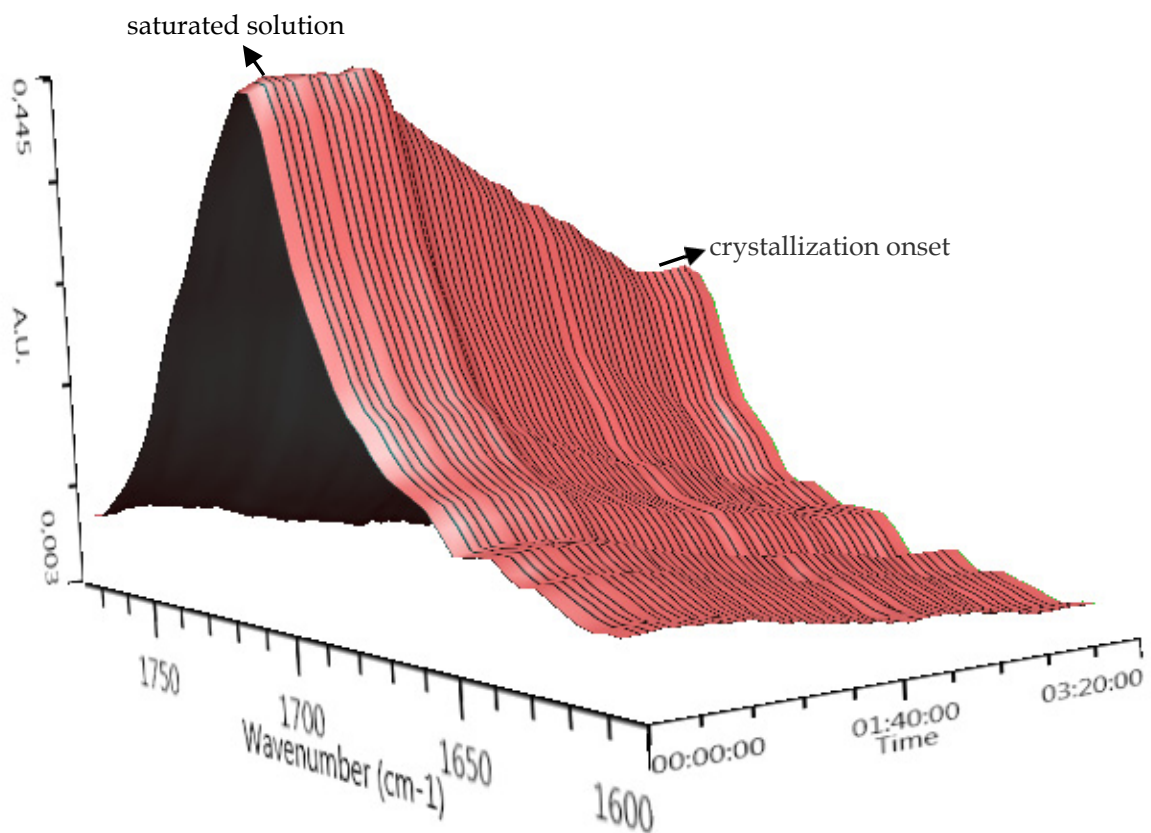
Fig. 12. Adipic acid carbonyl absorption variation measured in the interval of 1750-1600 \text{cm}^{-1} .
