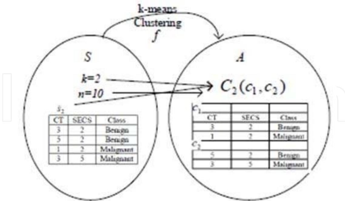
Figure 5. The mapping of function f s_2
