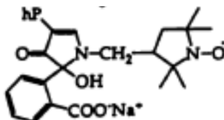
Figure 18. ((2-Carboxy)phenyl)-5-hydroxy-1-((2,2,5,5-tetramethyl-1-oxypyrrolidin-3-yl)methyl)-3-phenyl-2-pyrrolin-4-one sodium salt [30]
