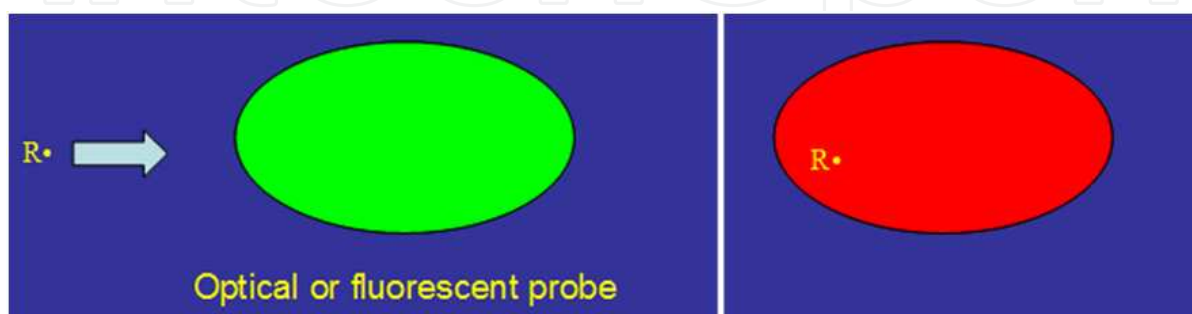
Figure 22. Schematic of the reaction of a colorimetric or fluorescent nitron spin trap with a radical
