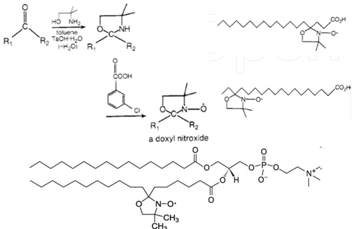
Figure 6. 16:0-7 Doxyl PC 1-palmitoyl-2-stearyl-(7-doxyl)-sn-glycero-3-phosphocholine.
