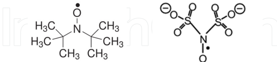
Figure 1. (left) di- t -butylnitroxide[2];(right) Fremy's salt [1]
