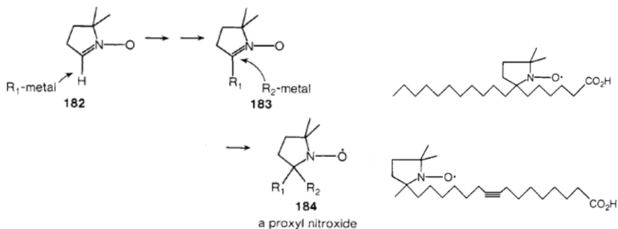
Figure 7. Synthesis of a proxyl nitroxide
