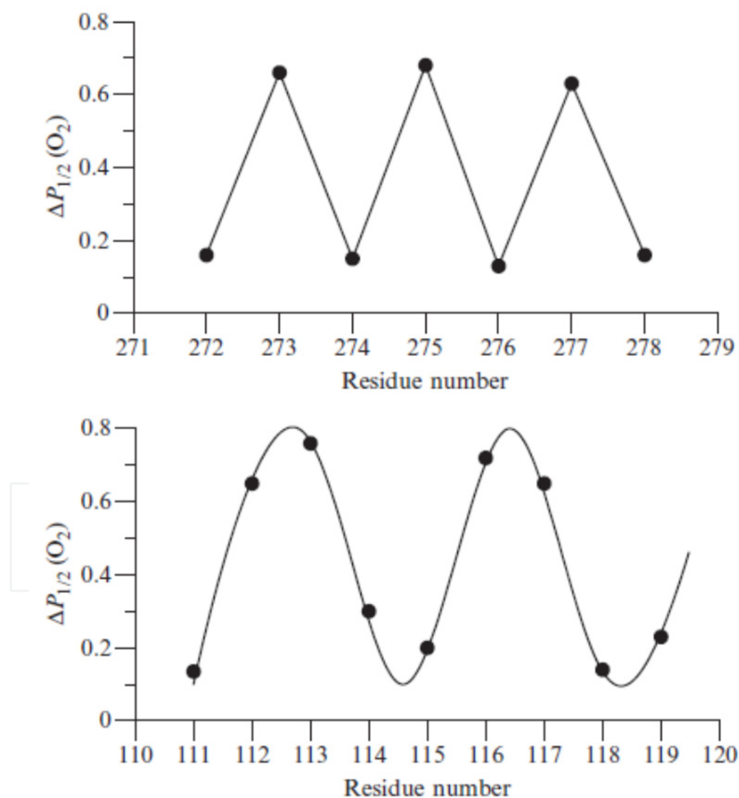
Figure 11. Idealized accessibility data plots indicating \beta -strand and \alpha -helical secondary structure. From [20] with permission
