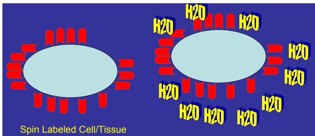
Figure 23. Schematic of a proton relaxation enhancement (PRE) spin labeled cell. Multiple paramagnetic labels are affixed to the cell surface by specific binding or covalent attachment. This results in a significantly enhanced PRE, which is detectable in MRI.
