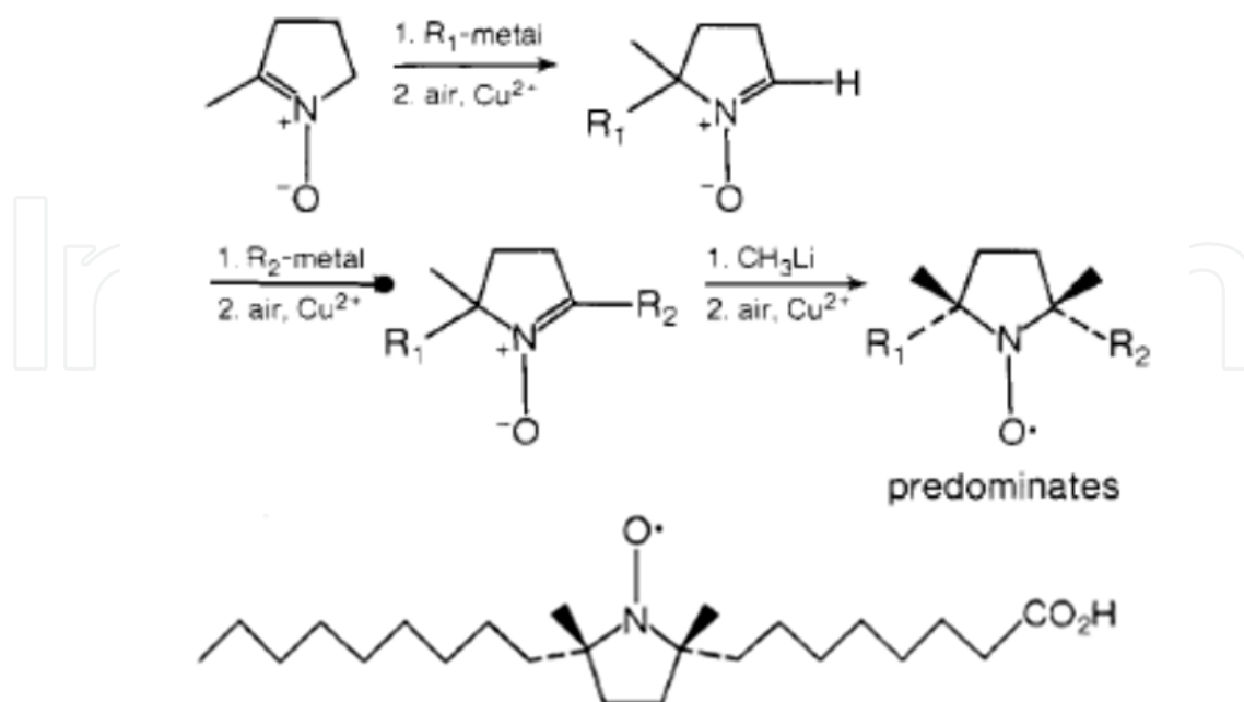
Figure 8. Synthesis of an azethoxyl nitroxide
