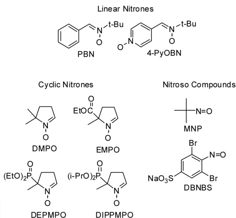
Figure 15. Structures of various spin trap types including second generation nitrones. Structure abbreviations: PBN \alpha -phenyl N-tert-butyl nitrone, 4PyOBN; DMPO 5,5-dimethylpyrroline N-oxide, EMPO 5-(ethoxycarbonyl)-5-methyl-1-pyrroline N-oxide, DEPMPO 5-(diethoxyphosphoryl)-5-methyl-1-pyrroline-N-oxide, DIPPMPO 5-diisopropoxy-phosphoryl-5-methyl-1-pyrroline-N-oxide, AMPO 5-carbamoyl-5-methyl-1-pyrroline N-oxide, MNP 2-methyl-2-nitroso propane, DBNBS 3,5-dibromo-4-nitrosobenzenesulfonate, CPCOMPO 7-oxa-1-azaspiro[4.4]non-1-en-6-one 1-oxide
