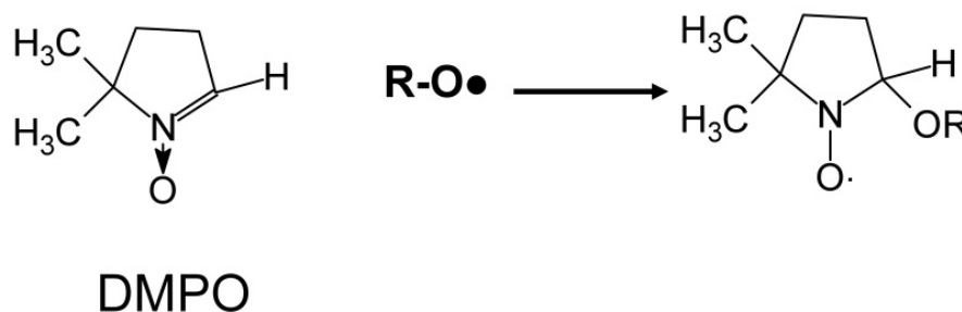
Figure 16. Reaction of DMPO with an oxyradical.
