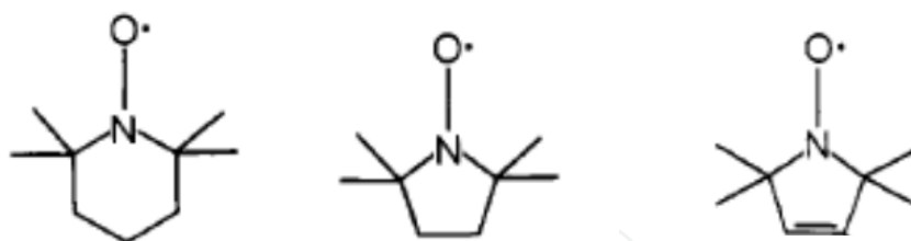
Figure 2. Piperidine, pyrrolidine and pyrroline nitroxides.
