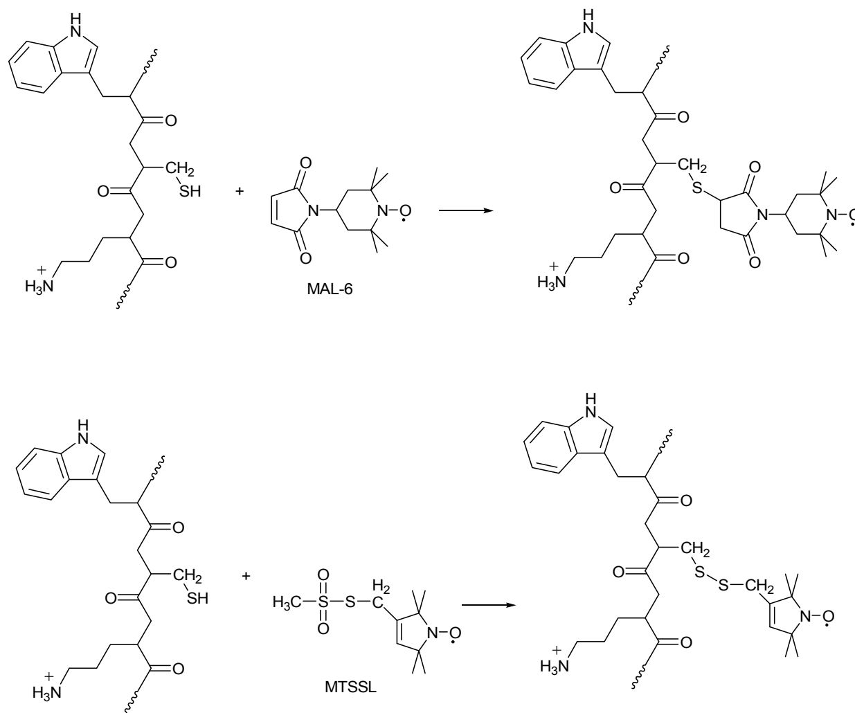
Figure 10. Comparison of thiol labeling reagents. The top reaction utilizes the NEM analog, which reacts irreversibly with the protein thiol group, but can also partially react with other nucleophiles. On the other hand, MTSSL reacts specifically with SH groups and can be reversed in the presence of another thiol reagent, such as mercaptoethanol or DTT. Adapted from [18] with permission
