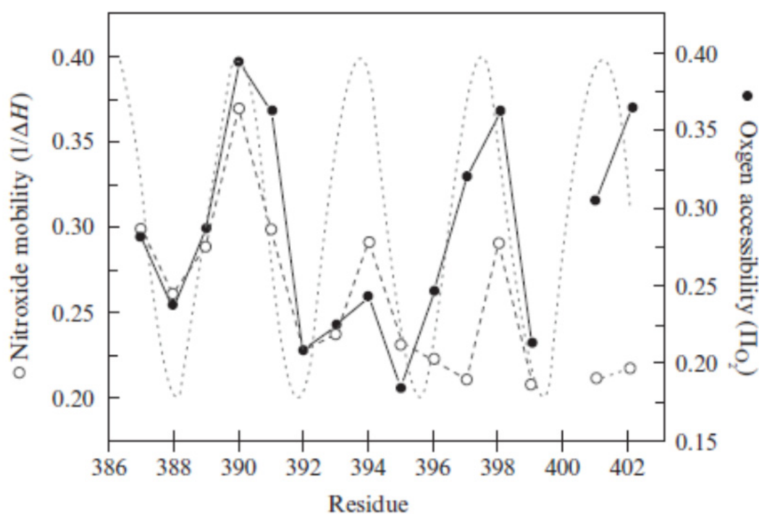
Figure 12. \Pi(O_2) (solid line) and 1/\Delta H (broken line) versus sequence position for the nitroxide-labeled single-Cys residues at positions 387-402 in lac permease. The dotted curve is that for a function of period 3.6, and comparison with the \Pi(O_2) and 1/\Delta H functions confirms that the data are consistent with an \alpha -helical structure. Ada[ted from [21] with permission.
