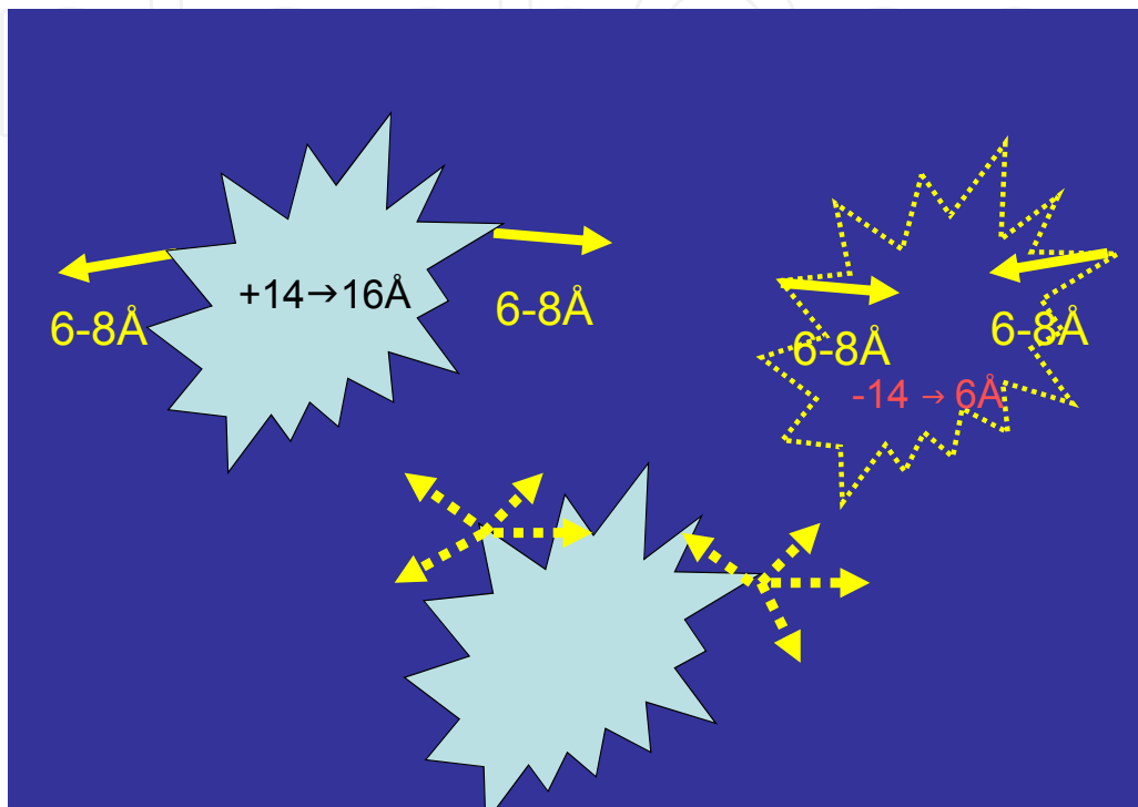
Figure 13. Uncertainty about spin label motion and orientation(s). The spin label ring can orient in several directions, depending on the flexibility of the tether. Ideally, one would like a rigid unique orientation, but the likelihood is not high.
