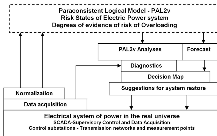
Figure 8. Paraconsistent logical model composed by risk evidence degrees obtained with values of current and voltage captures in the real electric power system.
