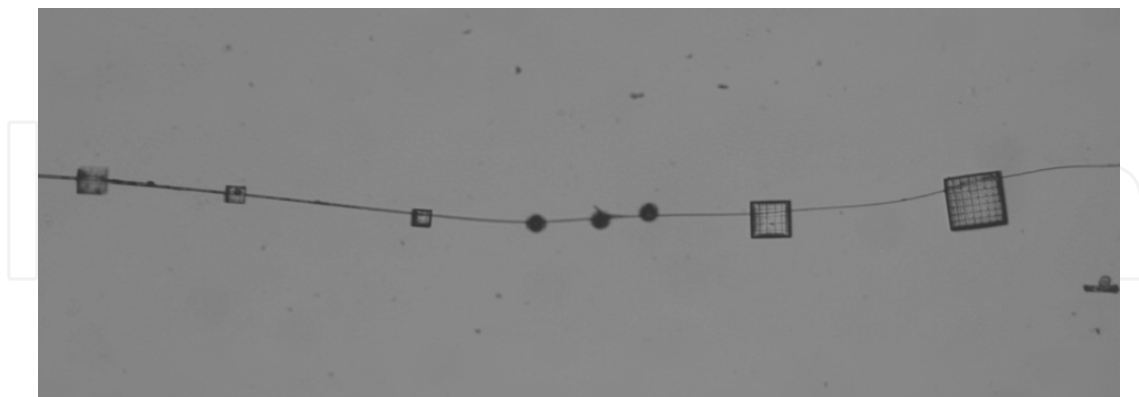
Figure 18. Transmission optical micrograph of a set of two-photon polymerized structures connected by tapered optical fibers.
