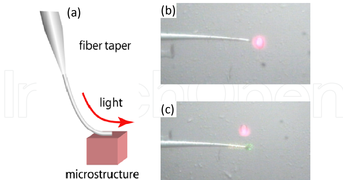
Figure 17. Excitation at 514 nm of a two-photon polymerized microstructure doped with rhodamine using silica tapered fiber. (a) Schematic view, (b) frontal excitation and (c) lateral excitation. (b) and (c) reprinted with permission from (Correa, et al.,2011). Copyright [2011], Springer Science+Business Media B.V.
