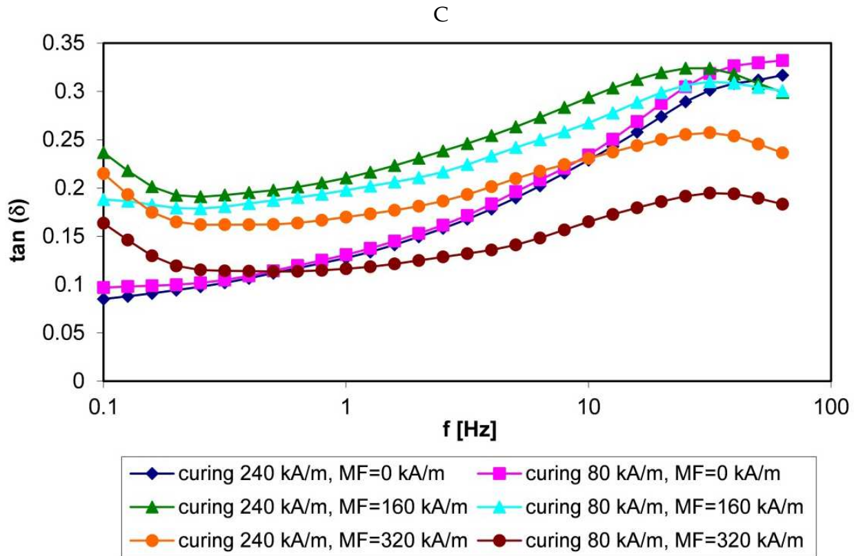
Figure 15. The change of rheological properties in the magnetic field as a function of frequency at a constant angular deformation of 0.1% for the MRE with PU matrix containing 11.5 vol.% Fe particles, cured in the 80 and 240 kA/m: A - storage modulus G' , B - the loss modulus G'' , C - damping factor \tan(\delta) .
