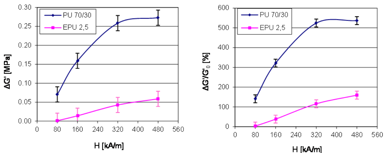
Figure 21. Absolute and relative MR effect of the MREs based on PU 70/30 and EPU 2.5 elastomers vs. the magnetic field strength (H).
