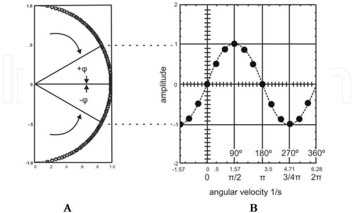
Figure 6. Dynamic measurements: a - deformation of the angle \phi , b - sinusoidal strain or stress.
