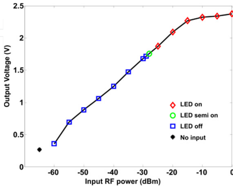
Figure 16. Measured output DC voltages of the RF power detection sub-module and the LED on/off states versus varying input RF power.
