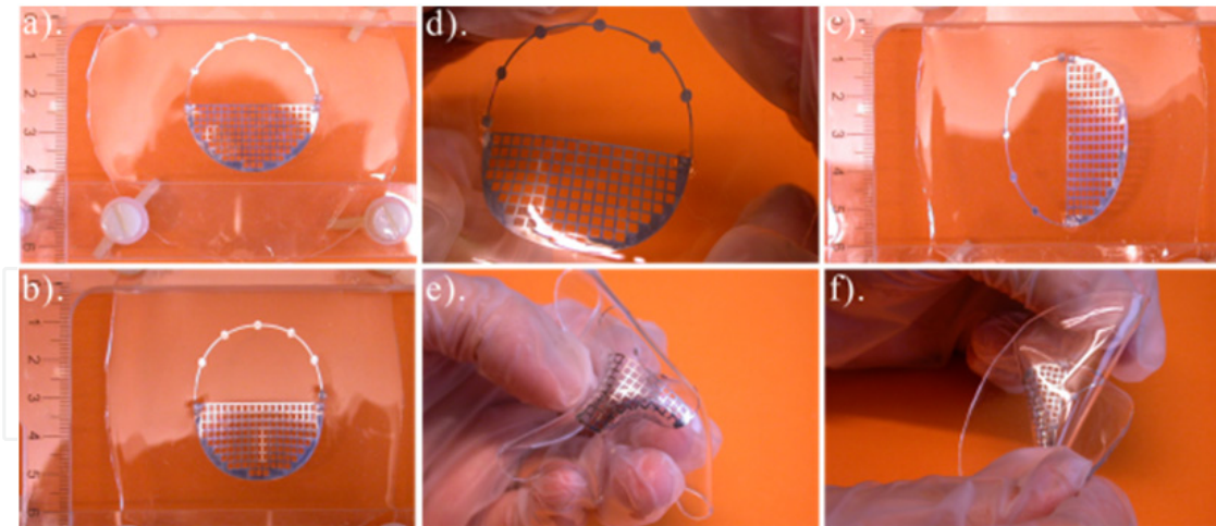
Figure 4. Photographs of the elastomeric fluidic unbalanced loop antenna: a). relaxed state, b). with 40% x -axis elongation, c). with 40% y -axis elongation, d). with biaxial elongation, e). bent state, and f). twisted state.
