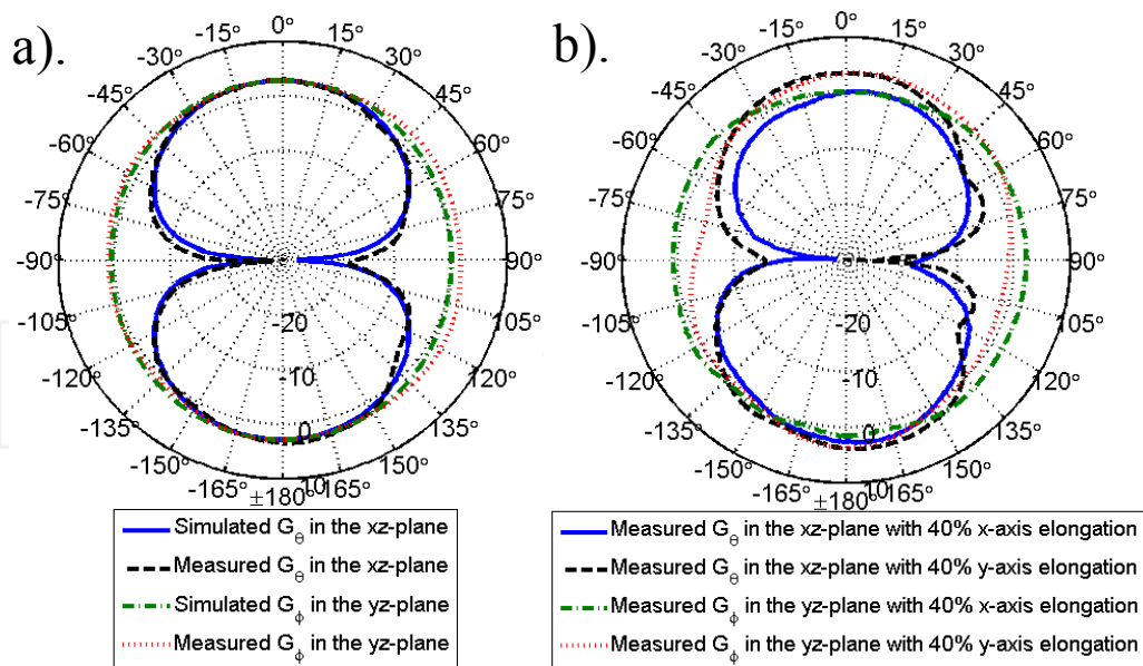
Figure 6. Simulated and measured radiation patterns of the a). relaxed and b). flexed antenna at 2.4 GHz. The corresponding coordinate system is depicted in Fig. 3. The antenna gain along \phi and \theta is defined as G_\phi and G_\theta , respectively.
