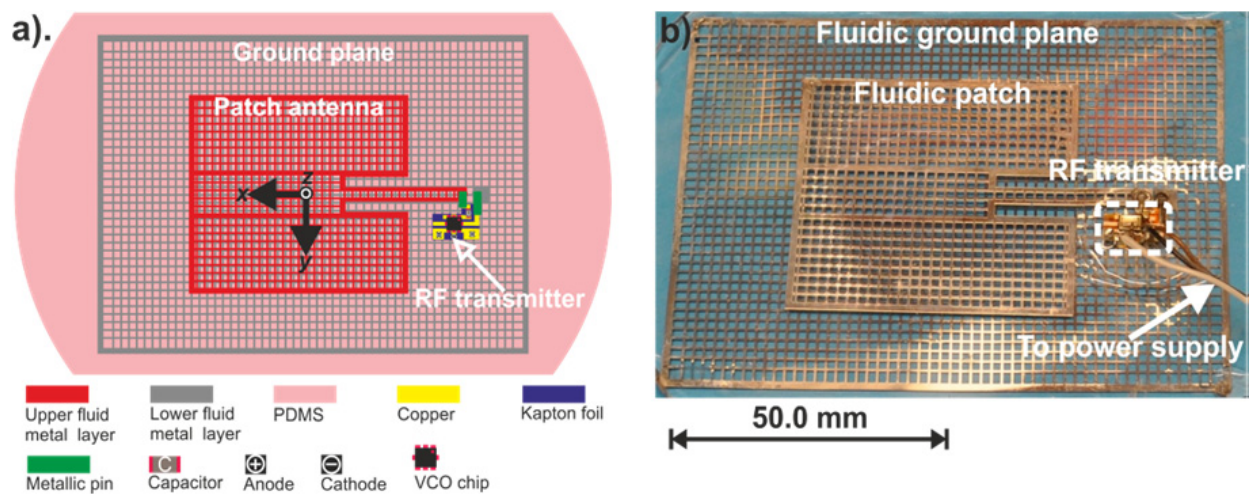
Figure 21. Demonstrated microfluidic reversibly stretchable wireless strain sensor: a). schematic illustration, and b). optical photograph of the resulting device.
