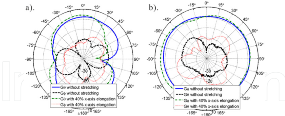
Figure 11. Measured a). xz - and b). yz -plane (according to the coordinate system in Fig. 7) radiation patterns at 2.5 GHz of the non-stretched and stretched antenna with 40% x -axis elongation.
