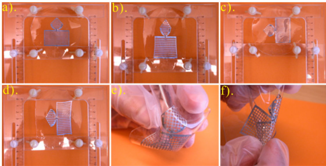
Figure 8. Photographs of the bendable, flexible, stretchable PICA: a). and c). relaxed state, b). strained antenna with 40% x -axis elongation, d). strained antenna with 40% y -axis elongation, e). folded antenna, and f). twisted antenna. The corresponding coordinate system is presented in Fig. 7.
