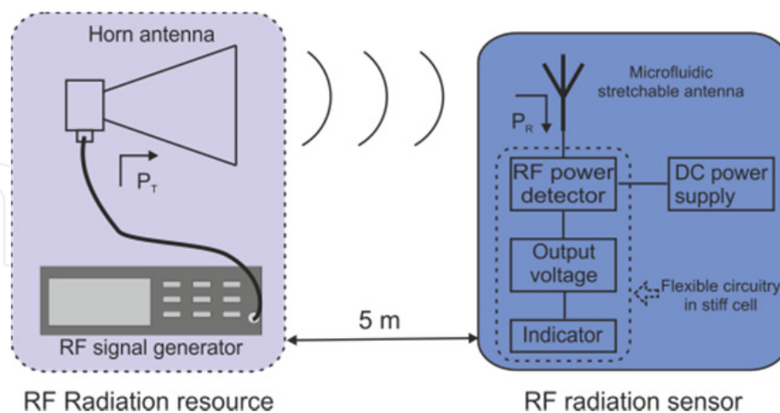
Figure 17. Schematic illustration of the RF radiation sensing demonstration setup.
