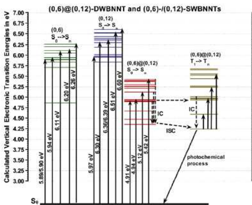
Figure 12. Calculated vertical electronic transitions, singlet-singlet ( S_0 \rightarrow S_n and triplet-triplet ( T_1 \rightarrow T_n ) for (0,6)&(0,12)-DWBNT and (0,6)- and (0,12)-SWBNTs. The vertically solid arrow indicated dipole allowed transitions. The broken arrows display possible internal conversion (IC) and intersystem crossing (ISC) processes.
