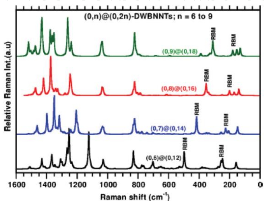
Figure 6. Calculated Raman spectra of the (0, n )&(0,2 n )-DWBNT, n = 0-9 .
