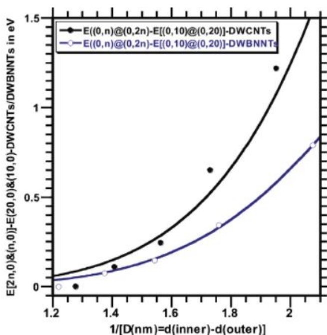
Figure 3. The diameter dependence of the curvature energies of the DWCNTs and DWBNNTs referenced to the global energies per hexagon of the (0,10)&(0,20)-DWCNTs/DWBNNTs is well fitted by a Lennard–Jones potential expression as given in Eqs. (3a) and (3b).
