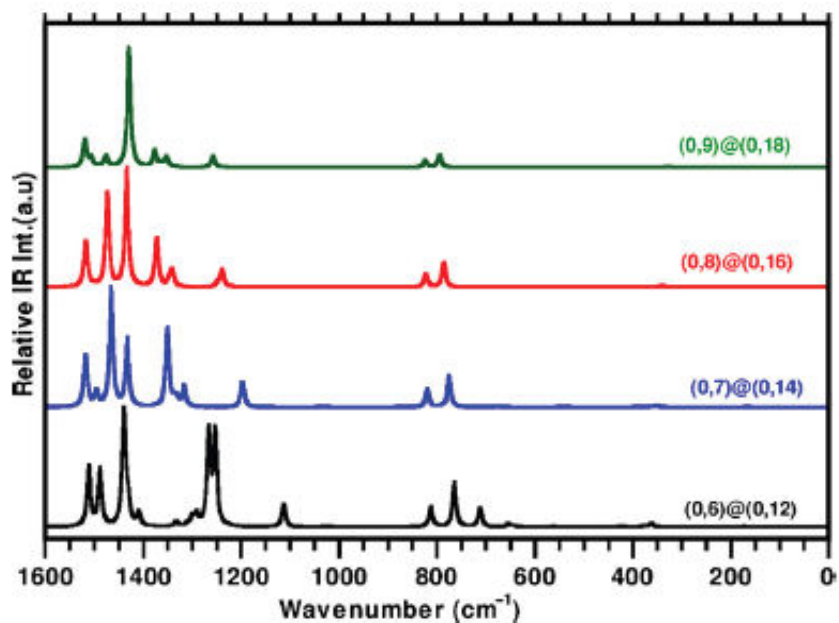
Figure 10. Calculated IR spectra of the (0,n)&(0,2n)-DWBNT, n = 6-9 .
