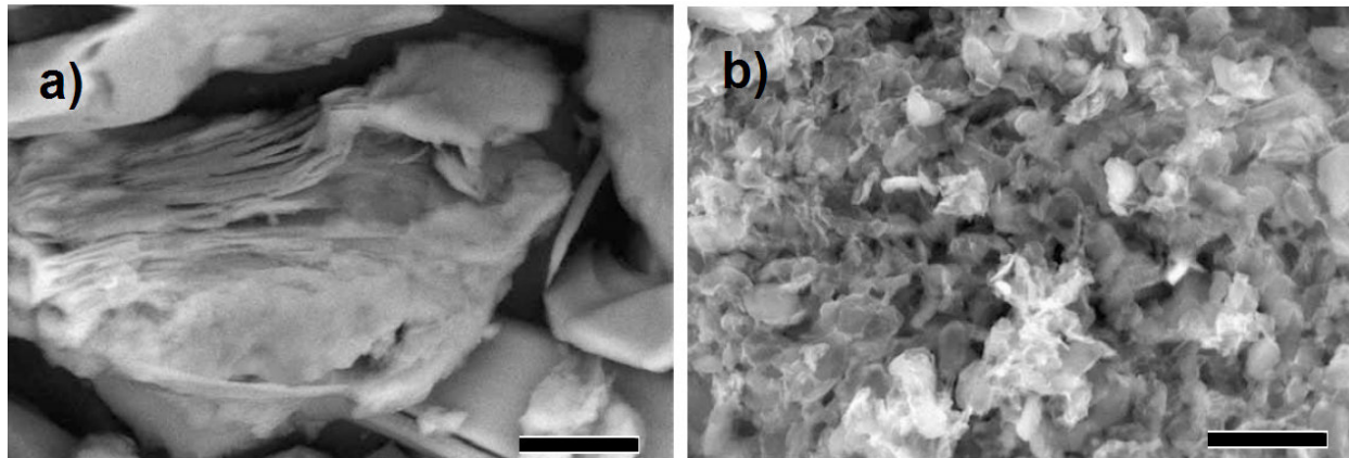
Figure 3. SEM images of original particle VER (a) and jet milled VER intercalated with ODA (sample 2). Bar shows 10 \mu\text{m} .
