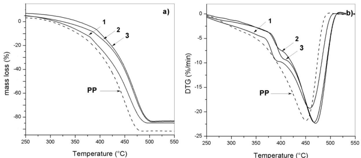
Figure 4. TG and DTA of ODA/VER nanofillers in PP.
