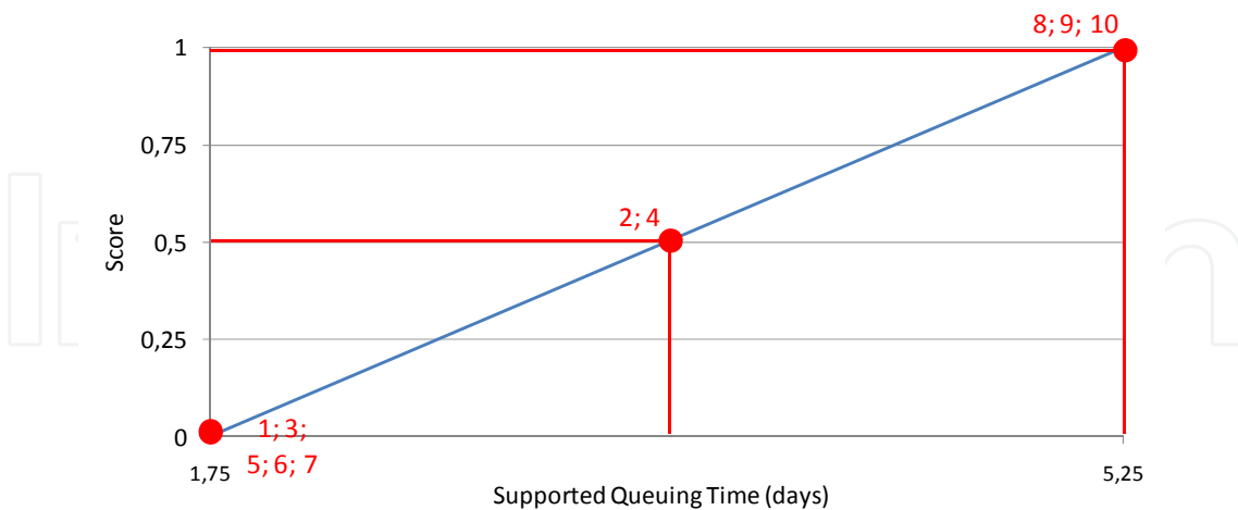
Figure 12. Determination of value function – supported queuing time.
