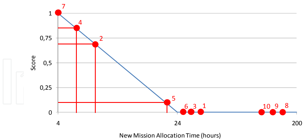
Figure 14. Determination of value function – new mission allocation time.
