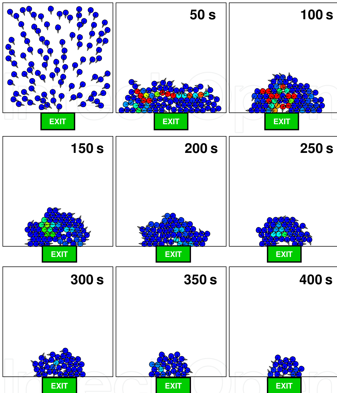
Figure 2. A novel feature of the current approach where collision forces developed due to human-human collisions during the evacuation process can be predicted by the algorithm.
