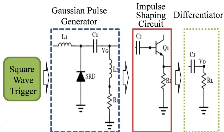
Figure 3. Schematic of proposed monocyte pulse generator.
