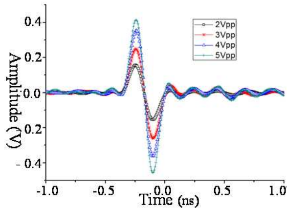
Figure 9. Measurement results with variations in triggering amplitude.
