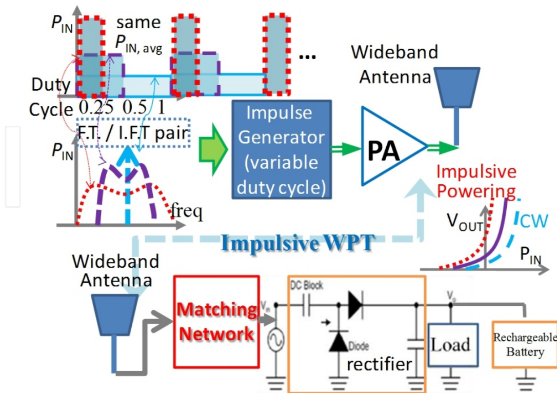
Figure 1. Schematic of proposed monocycle pulse generator.
