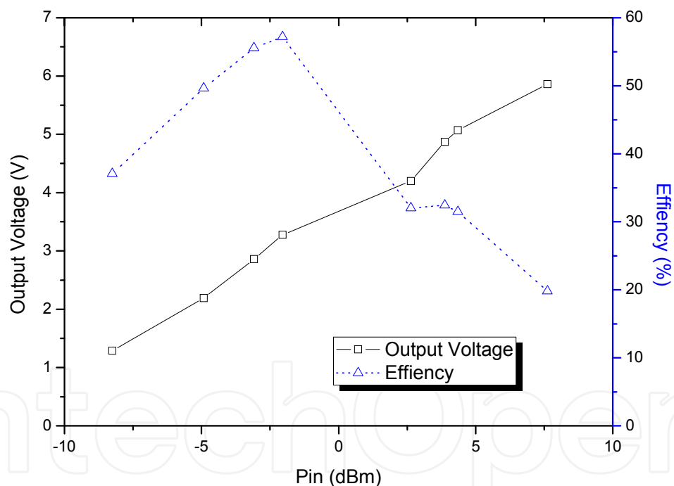
Figure 11. The performance of the wideband recharging for the resistive load of 30 k \Omega .
