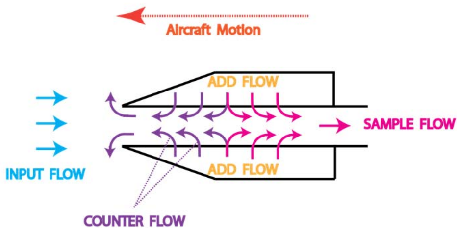
Figure 1. a: Flow schematics within the pumped counterflow virtual impactor (PCVI). Input flow carries the condensation nuclei and interstitial particles (non-activated aerosol particles). The large particles that have sufficient inertia to cross the streamlines enter the counterflow; these particles that
