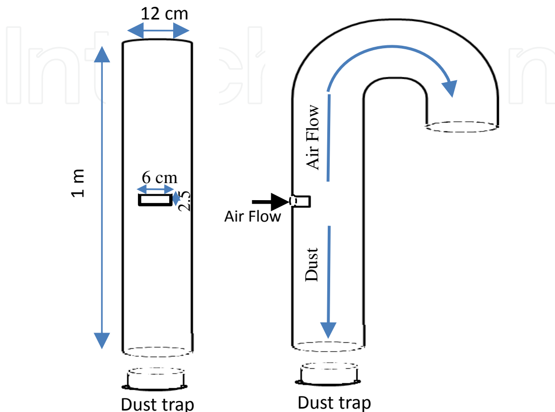
Figure 6. Schematic diagram of the dust sampler system.
