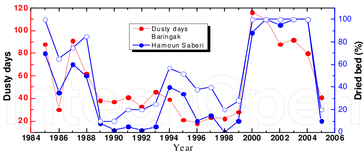
Figure 10. Yearly variability of the dusty days (visibility \leq 2 km) over Sistan region with association to percentage of Hamoun dried beds (1985-2005). The lower coverage of the Hamoun Basin by water (high percentage of dried beds) corresponds to higher number of dusty days over Sistan region.
