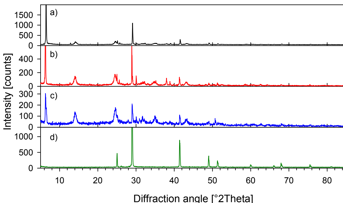
Figure 3. XRD investigation of the stability of \text{NaBH}_4 -gel under open conditions: a) directly after precipitation and drying for two hours, b) after 10 days, held under open conditions and c) after 4 weeks under open conditions. The pattern of pure \text{NaBH}_4 -salt (dried at 110^\circ\text{C} ) is included for comparison (d).
