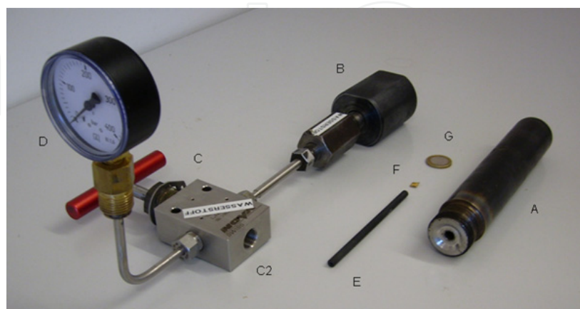
Figure 18. Equipment for hydrogen pressure experiments: Autoclave (A), connection piece (B) between autoclave and closing device with three-way switch (C) with opening to the outer hydrogen bottle (C2) and to the manometer (D). Filling piece (E) and Au capsule (F).
