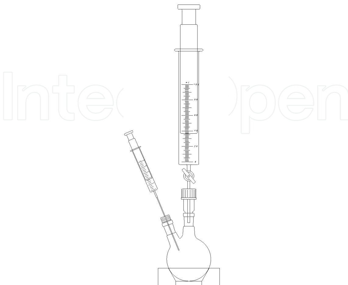
Figure 6. Apparatus as used for measuring gas release
