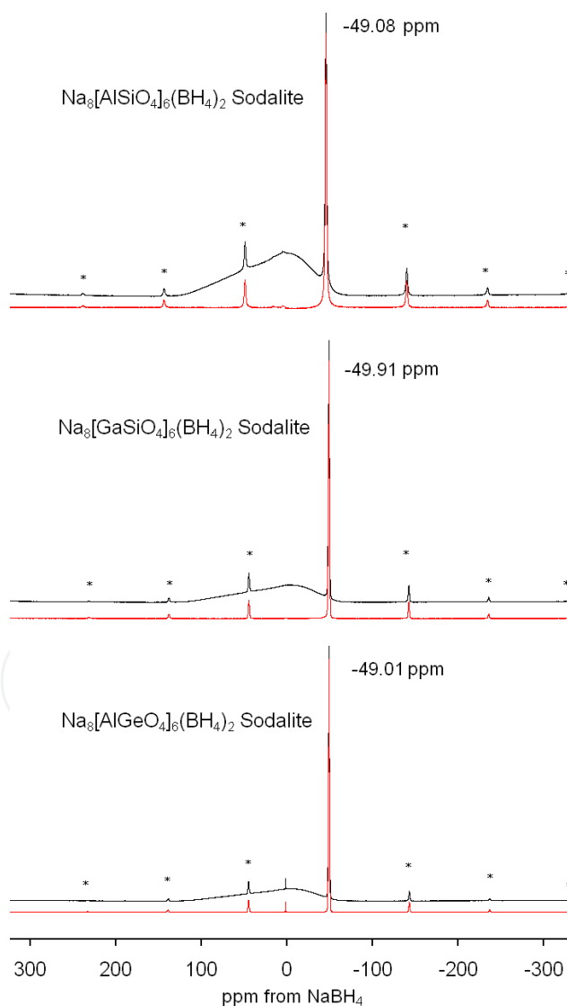
Figure 15. ^{11}\text{B} MAS NMR spectra of the microcrystalline \text{NaBH}_4 sodalites; asterisks mark the spinning side bands, lower spectra are given after the subtraction of the probe background (after [65]).
