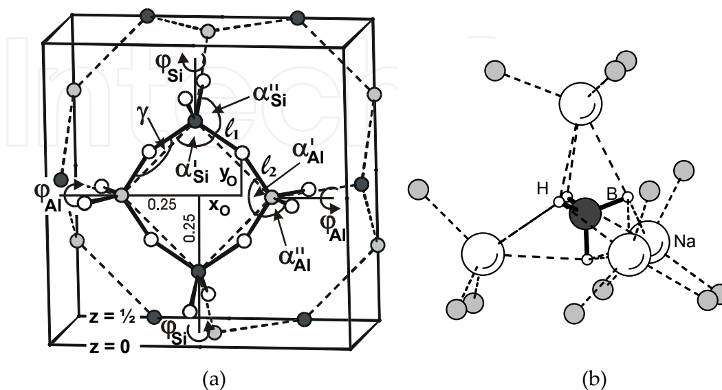
Figure 14. a, left) Perspective view of one half of the sodalite cage (after [50]) depicting sixring and fourring windows (dashed lines) and denoting bond lengths ( l_1 , l_2 ) and tetragonal tetrahedral distortions ( \alpha' , \alpha'' ), tilt angles ( \phi ) and oxygen coordinates of the framework ( x_0 , y_0 , z_0 ). Note z_0 > 0 determines \phi > 0 and z coordinate shifted by 1/2 compared to values given in Tab. 2. b, right) Coordination of the non-framework atoms in the microcrystalline \text{NaBH}_4 sodalite together with three oxygen atoms of the framework around each sodium atom [17].
