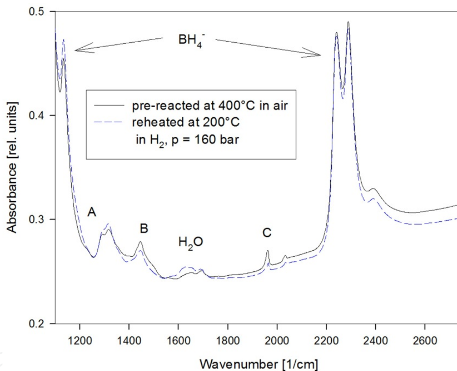
Figure 30. IR absorption spectra of microcrystalline \text{BH}_4^- -aluminosilicate sodalite sample with addition of Pt pre-reacted for 1 h at 400°C in air and reheated for 3 h in 160 bar \text{H}_2 at 200°C, after [25] (compare text).
