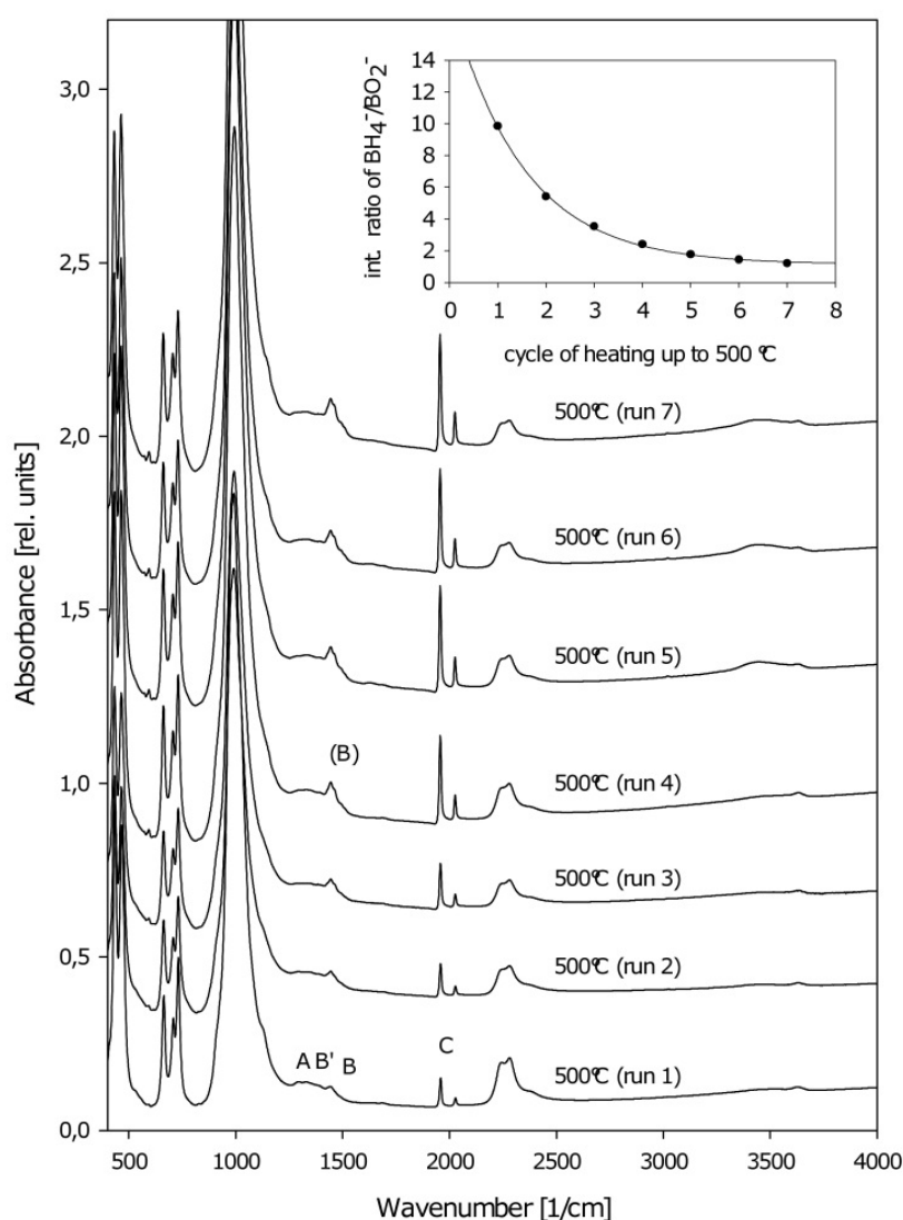
Figure 21. IR-absorption spectra of BH 4 -sodalite sample of nominal composition Na 8 (AlSiO 4 ) 6 (BH 4 ) 2 (as synthesized) after thermal treatment at 500°C (heating rate 2°C/min, 0.5 h holding time, flowing He 20 ml/min). Spectra were taken after each cycle and exposure the sample to atmospheric conditions for 24 h by KBr method for a part of the sample. The remaining sample was given to the next thermal treatment.
