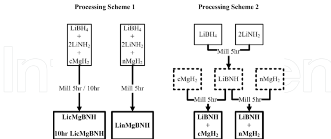
Figure 11. Processing schemes of synthesizing complex hydrides \text{LiBH}_4/2\text{LiNH}_2/\text{nanoMgH}_2 via reactive gas milling.
