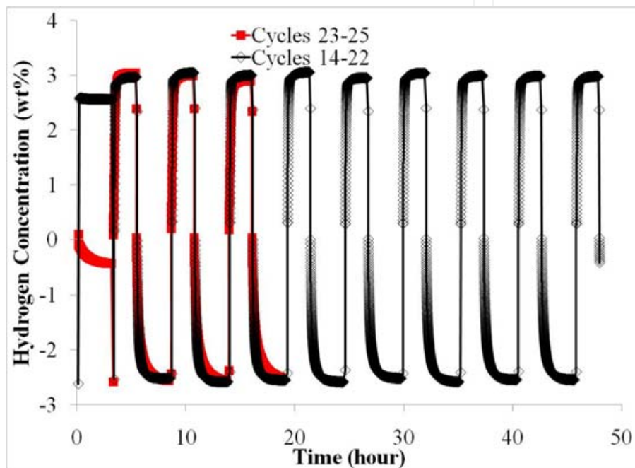
Figure 9. Hydrogen sorption kinetics in PANI-NF-CM.
