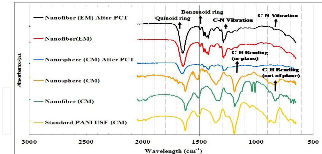
Figure 4. FTIR spectra of polyaniline nanofibers and nanospheres.
