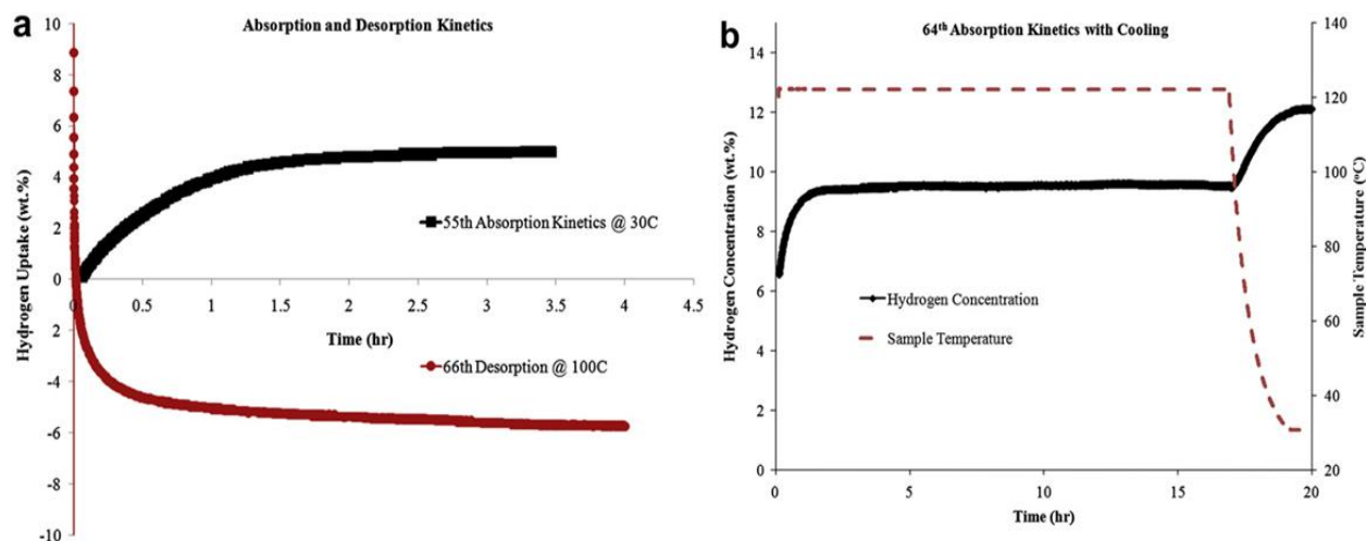
Figure 8. Hydrogen sorption kinetic curves of PANI-NF electrospun samples at different cycles.
