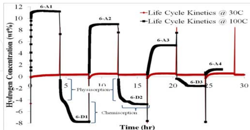
Figure 6. Hydrogen sorption kinetics in PANI-NF-ES.
