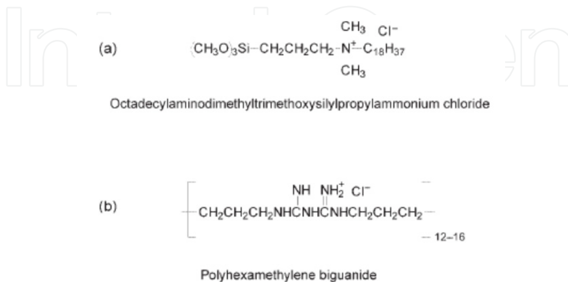
Fig. 12. Bound antimicrobials
