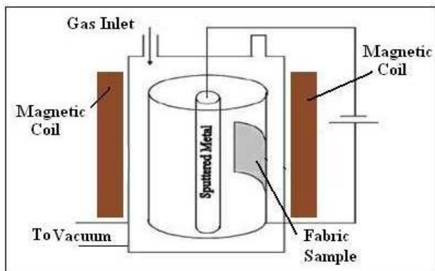
Fig. 3. The schematic view of Plasma sputtering system
