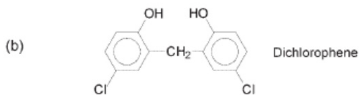
2,2'-Dihydroxy-5,5'-dichlorodiphenyl methane
