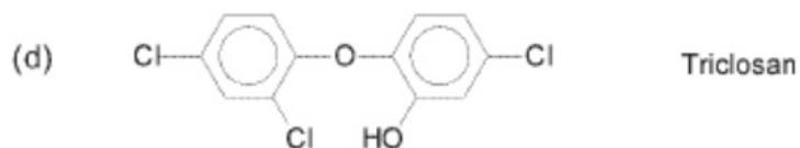
2,4,4'-Trichloro-2'-hydroxydiphenyl ether
