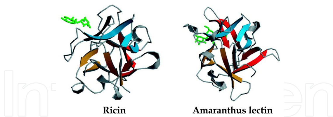
Fig. 4. The \beta -trefoil folds illustrated by the first domain of the subunit ricin (in complex with lactose), the first domain of amarantin (in complex with the T-antigen) In each case, for clarity, only a single \beta -trefoil domain is shown in an identical orientation, although each protein is a multidomain as well as a multimeric protein. Bound carbohydrate is shown in green ball-and-stick (Loris, 2002).
