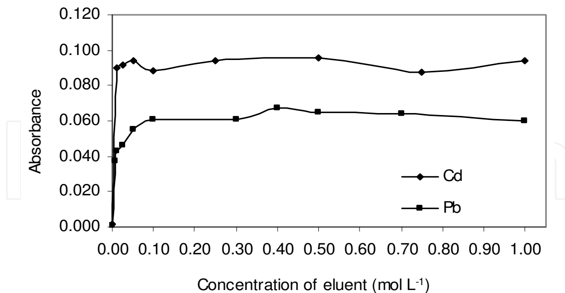
Figure 7. Influence of eluent concentration on the determination of Cd and Pb using solid phase extraction.
