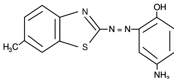
Figure 1. Proposed structure of Me-BTAP.
