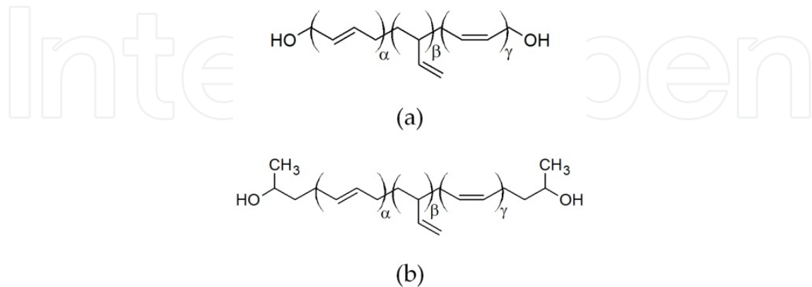
Figure 11. Molecular structure of (a) free radical HTPB, and (b) anionic HTPB prepolymer (Krasol LBH-3000)
