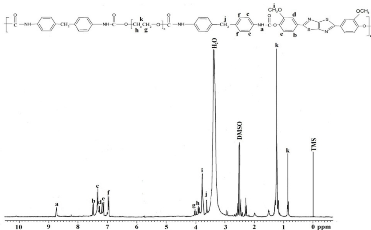
Figure 2. 1 H-NMR spectrum of LCPUE VIIa
