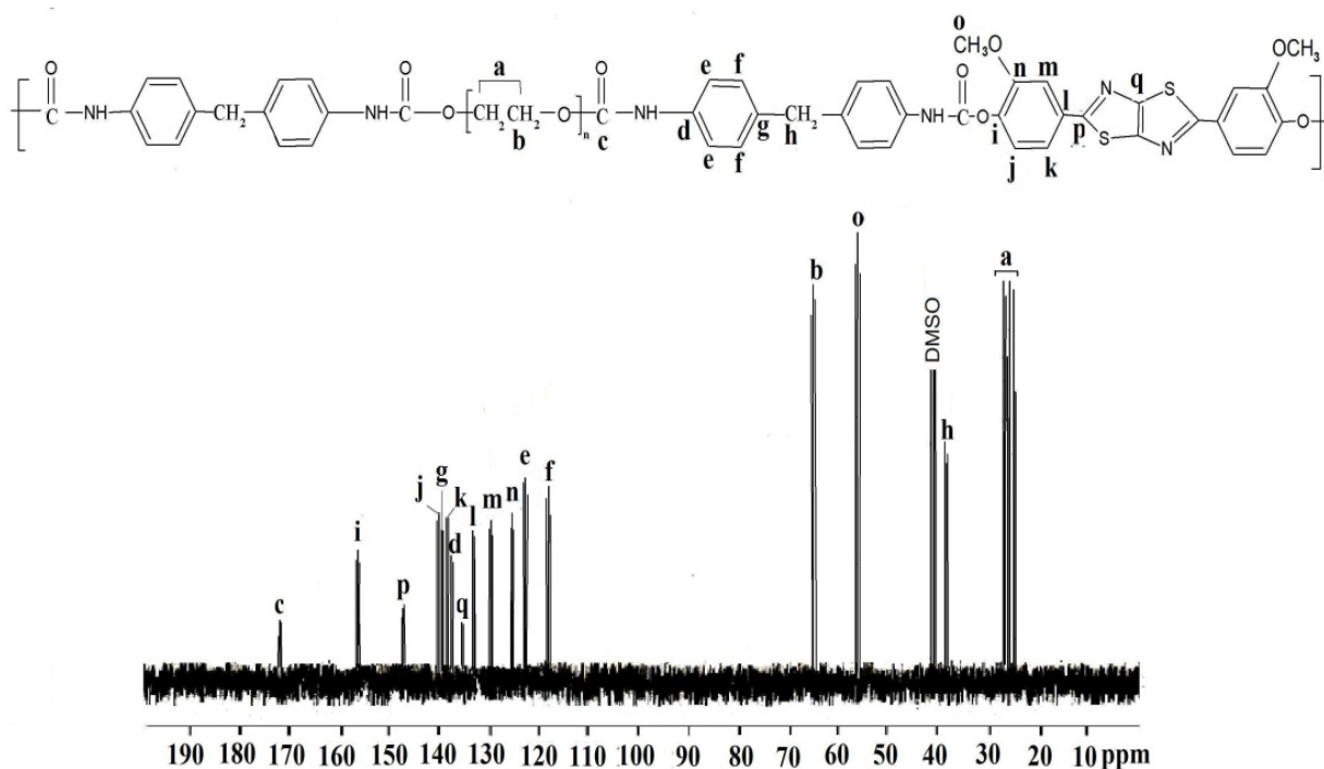
Figure 3. 13 C-NMR spectra of LCPUE VIIa
