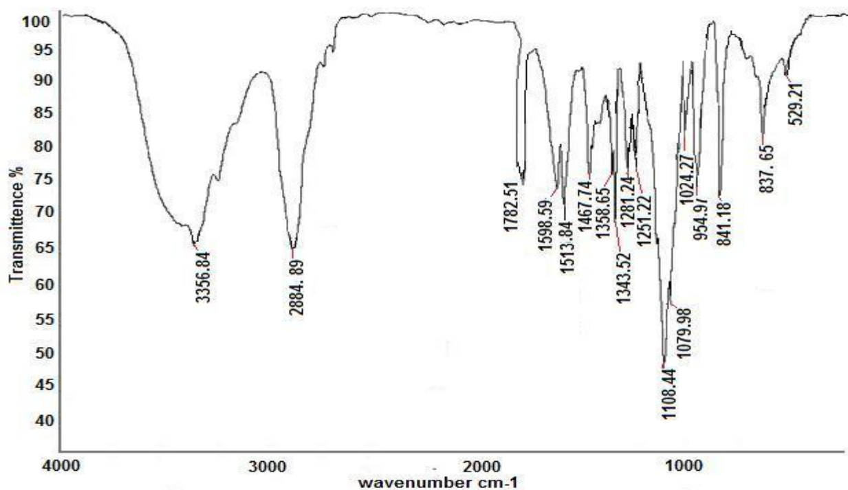
Figure 1. FTIR spectrum of LCPUE VIIa
