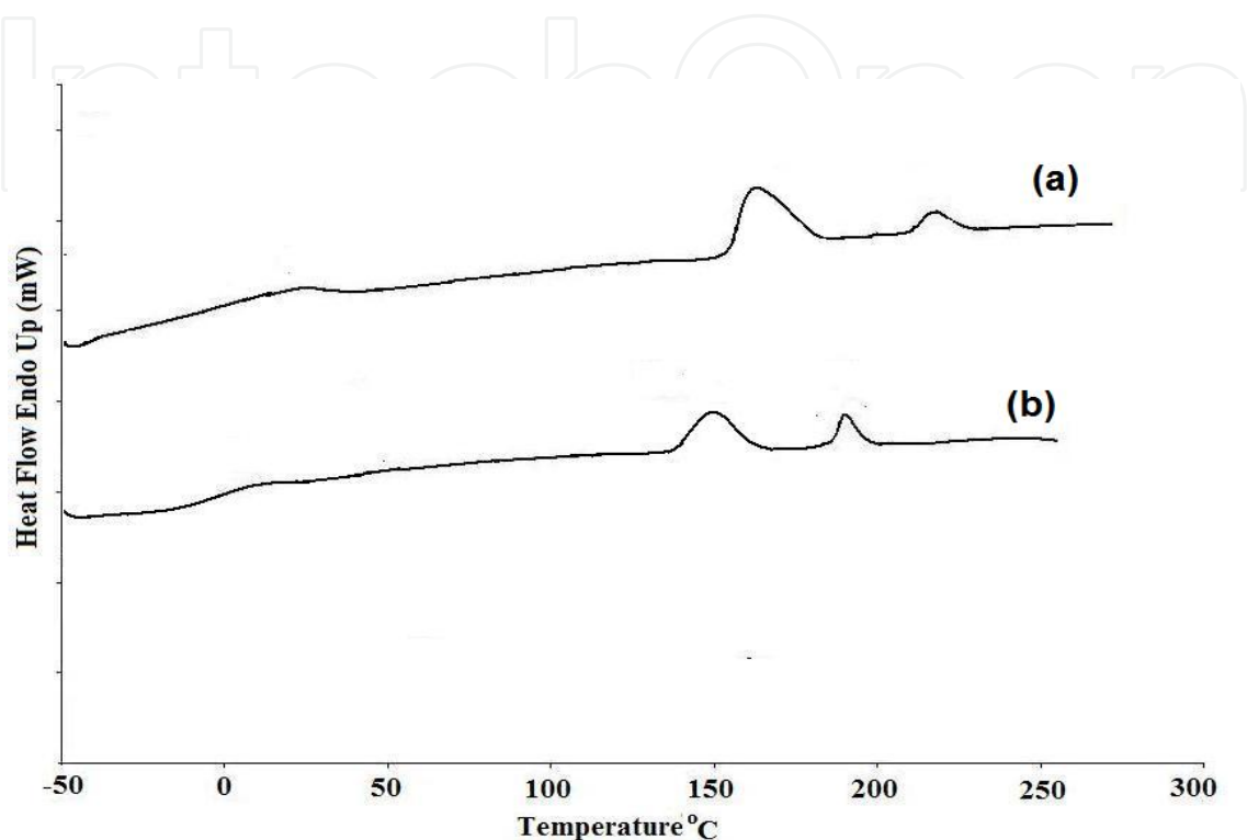
Figure 4. DSC traces of (a) LCPUE VIa (b) LCPUE VIIa
